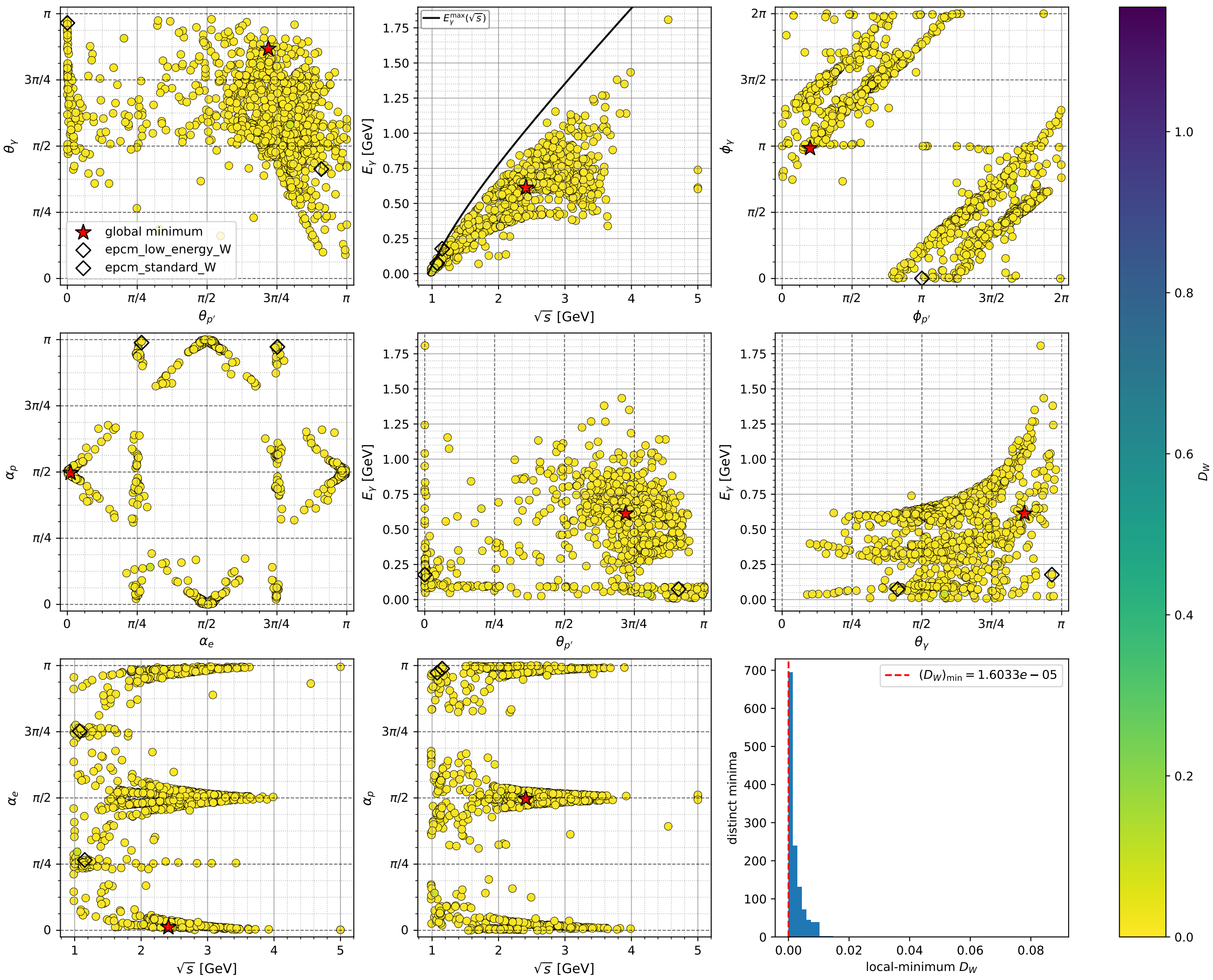
electron: all 1268 distinct gradient-search local minima of D_W
