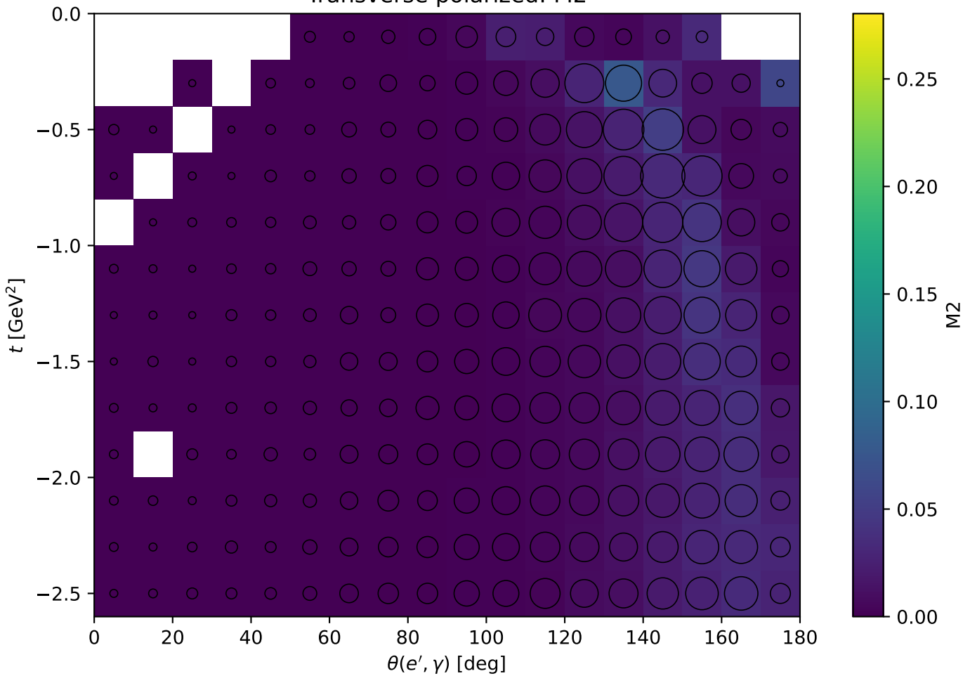
Transverse polarized: M2
