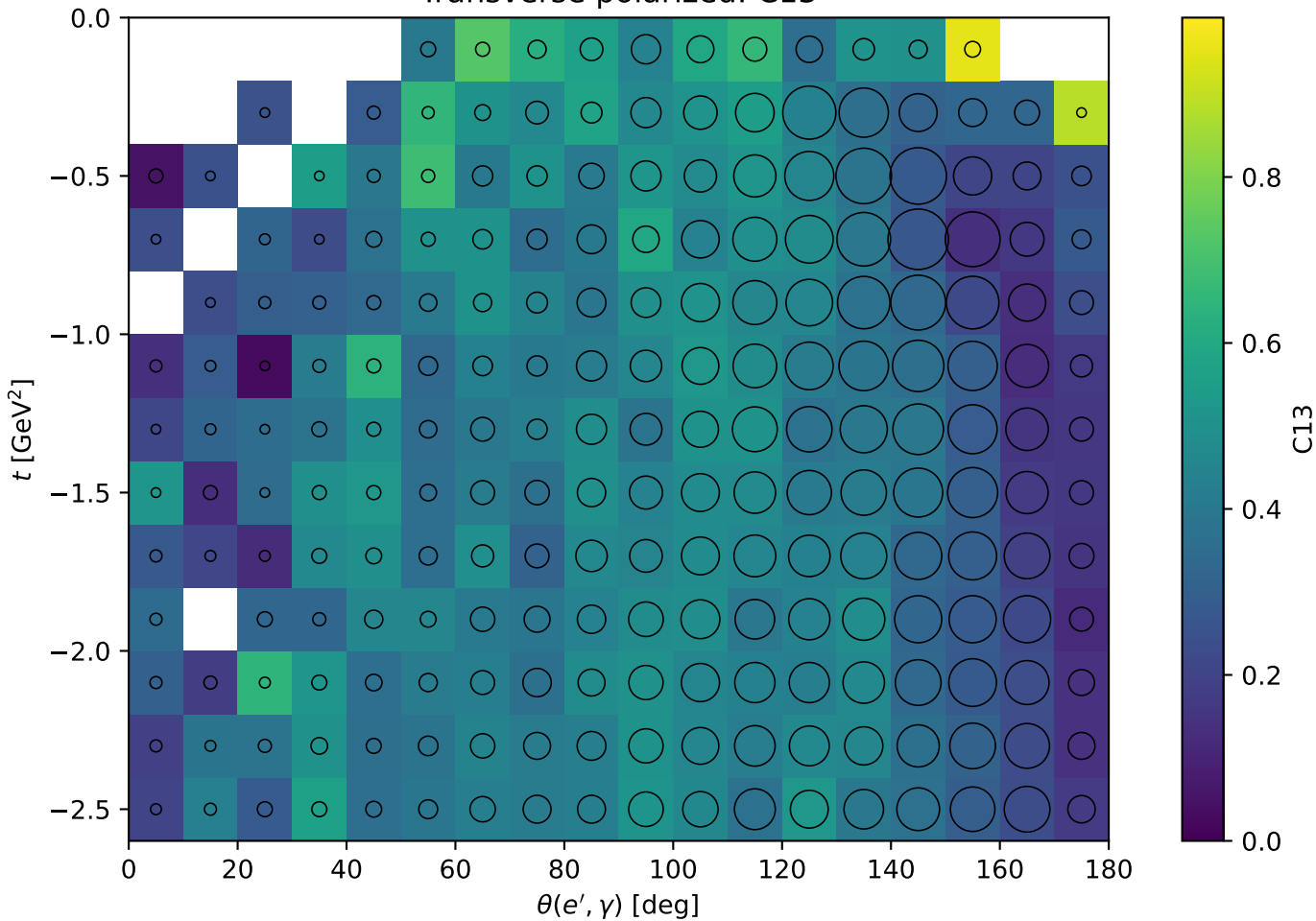
Transverse polarized: C13
