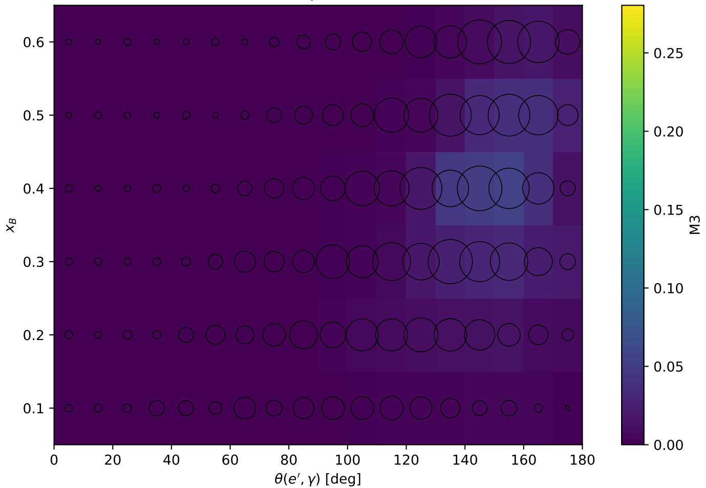
Transverse polarized: M3
