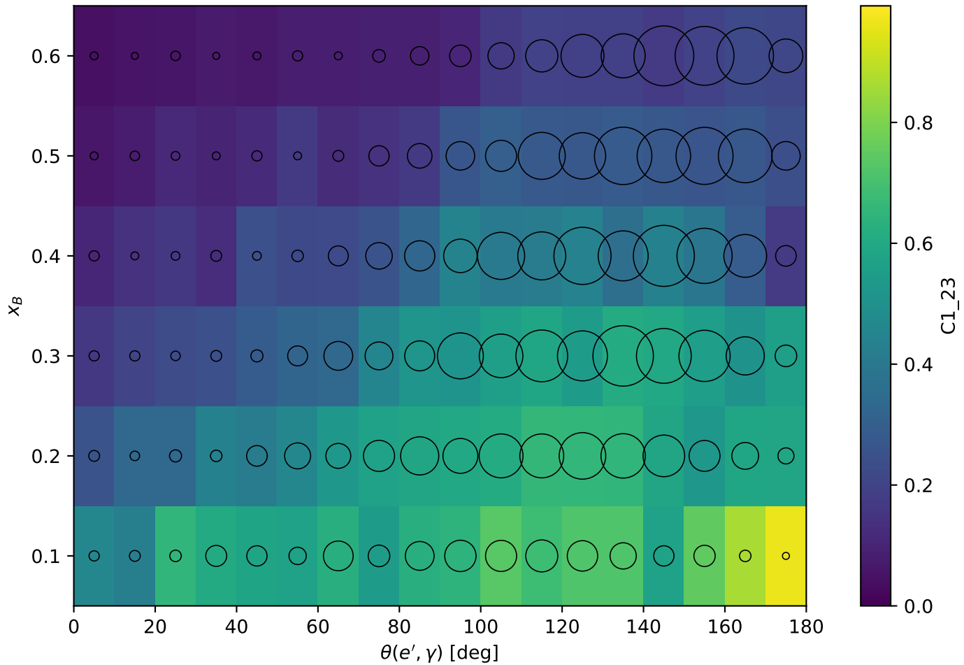
Transverse polarized: C1_23
