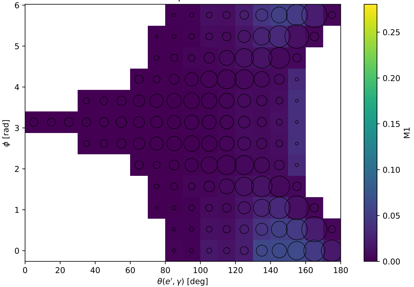
Transverse polarized: M1
