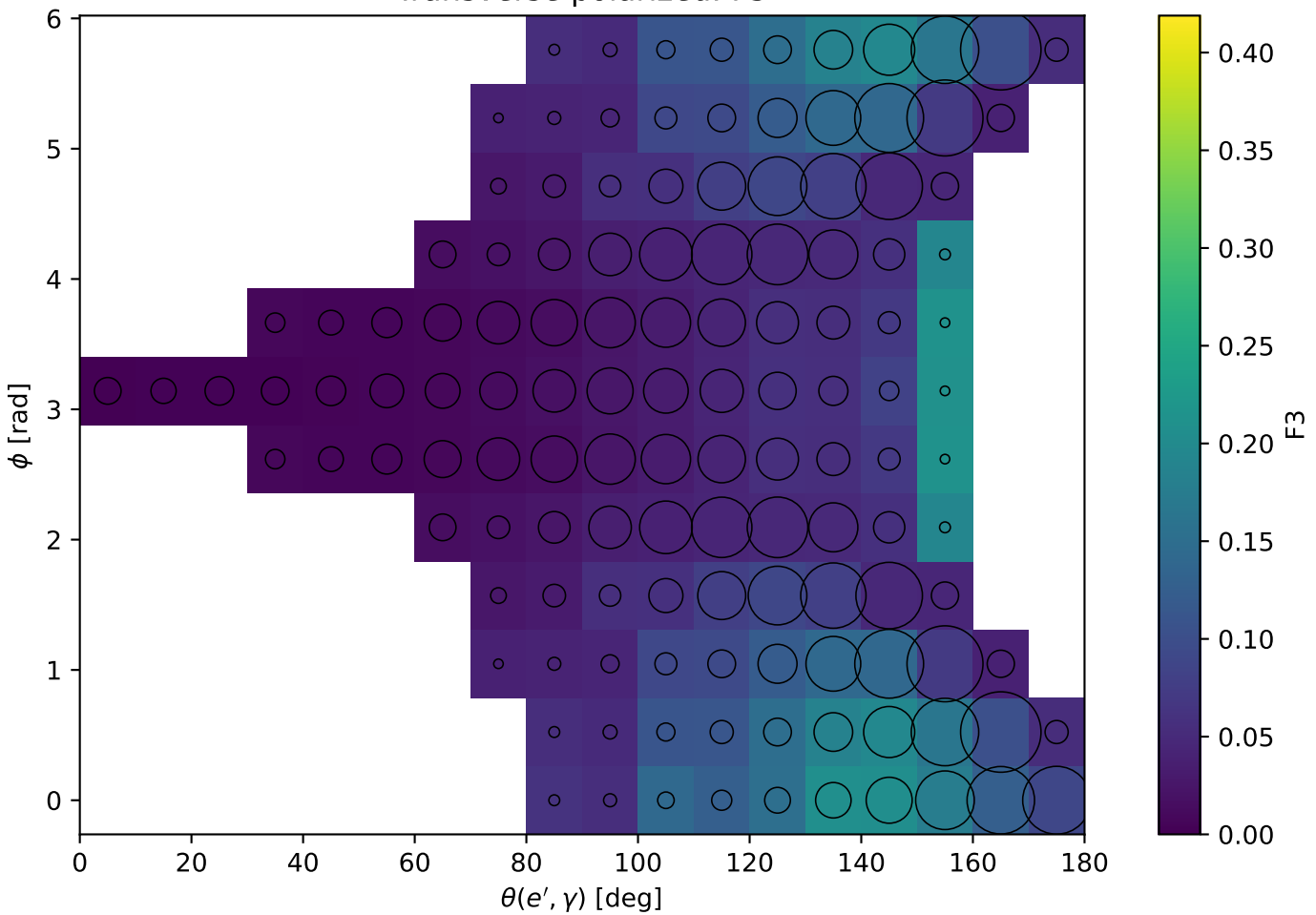
Transverse polarized: F3
