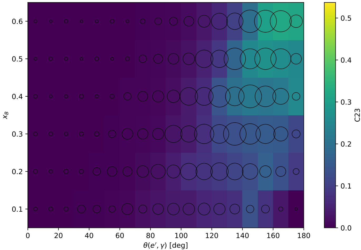
Transverse polarized: C23
