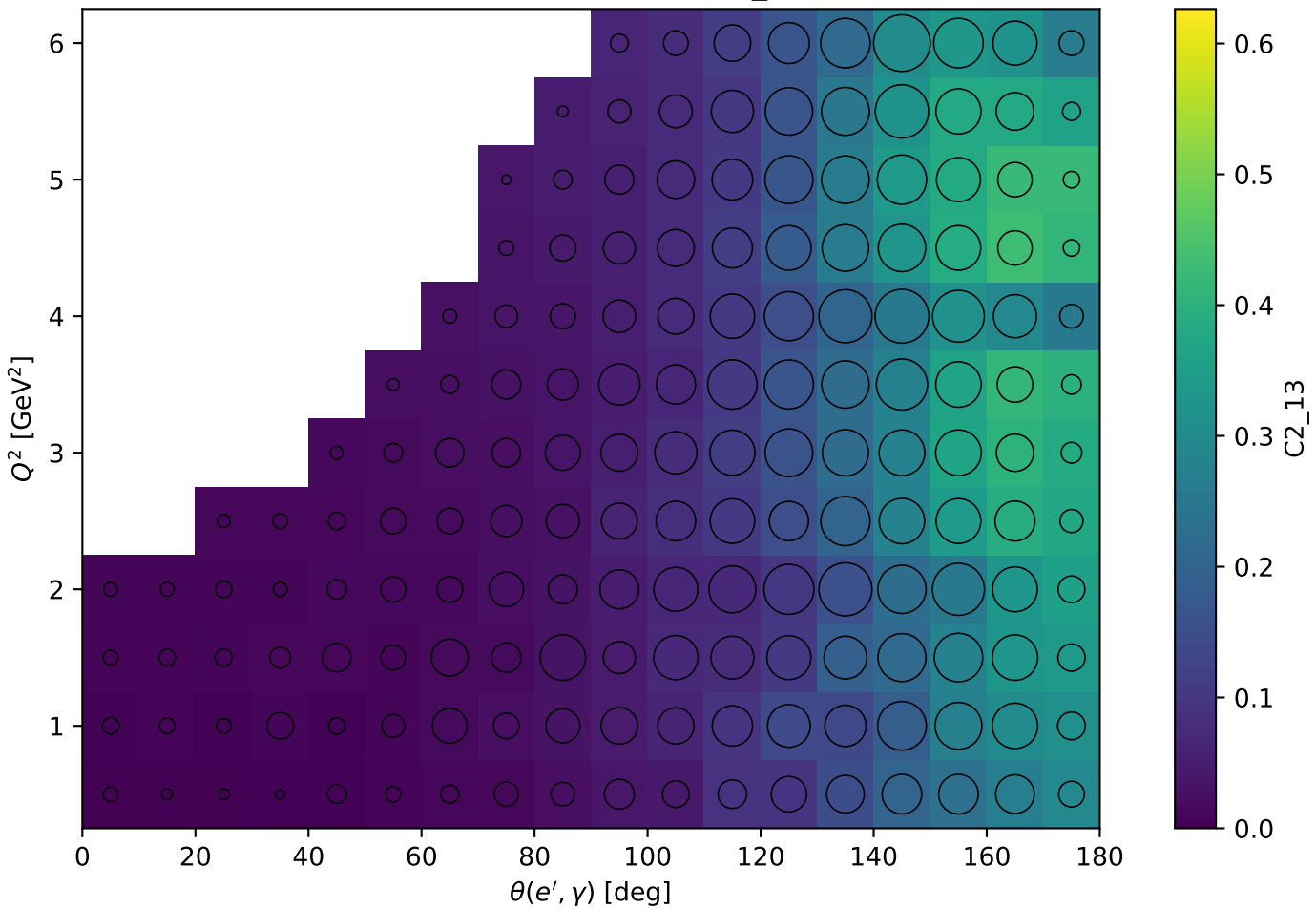
Transverse polarized: C2_13
