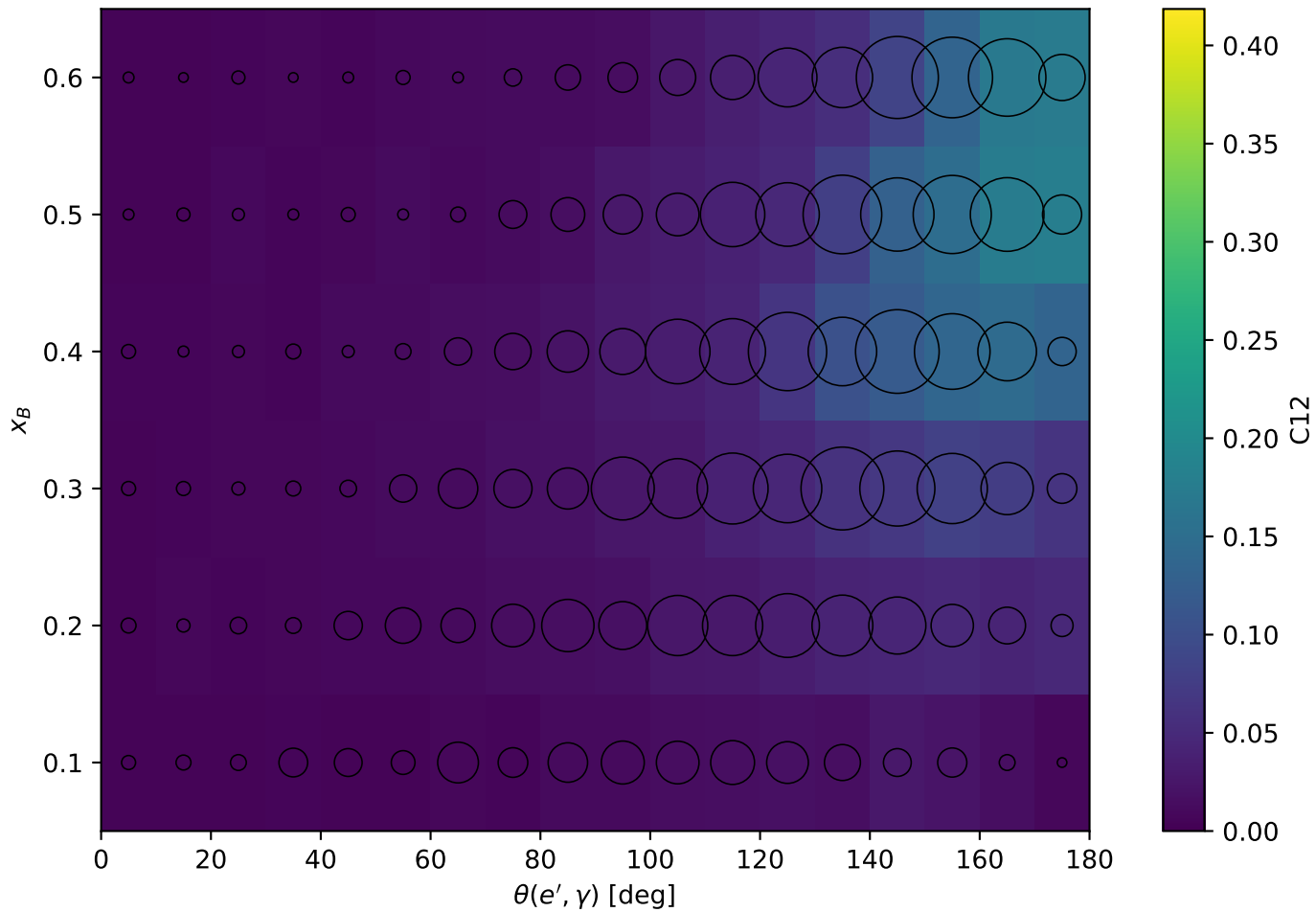
Transverse polarized: C12
