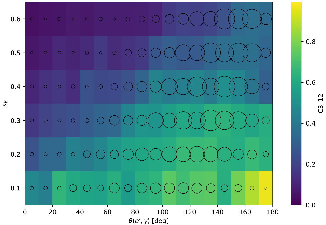
Transverse polarized: C3_12
