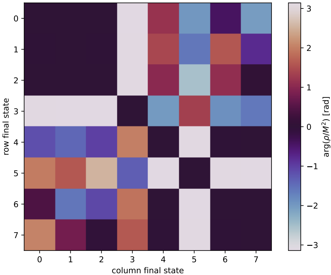
\arg(\rho/M^2) at unpolarized, Q2=6, phi=0
