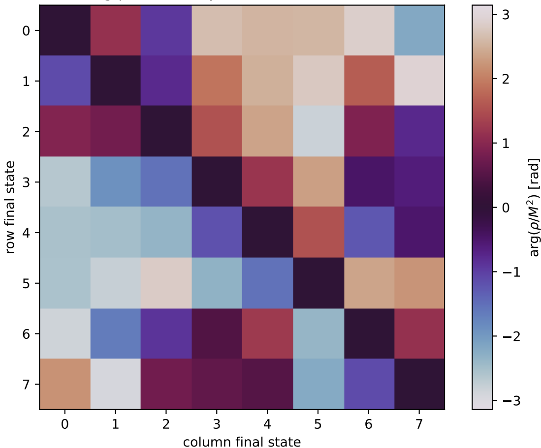
\arg(\rho/M^2) at unpolarized, Q2=2, t=-0.8
