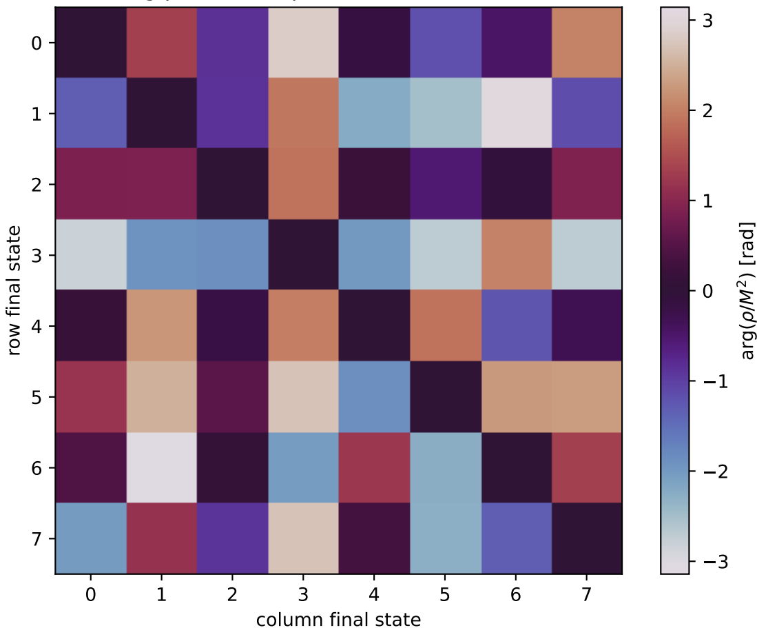
\arg(\rho/M^2) at unpolarized, Q^2=2.5 , t=-1
