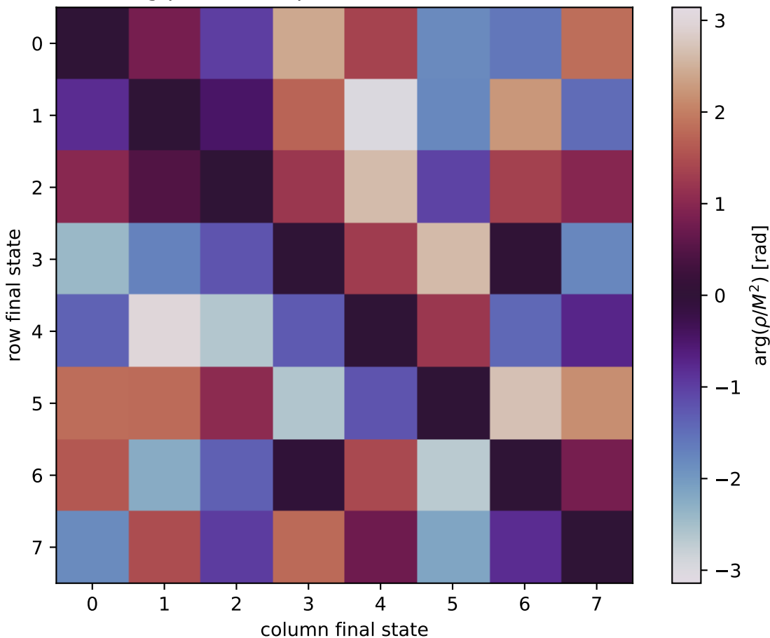
\arg(\rho/M^2) at unpolarized, Q^2=3 , t=-0.4
