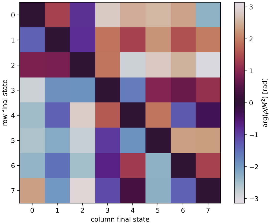
\arg(\rho/M^2) at unpolarized, Q2=3, t=-0.9
