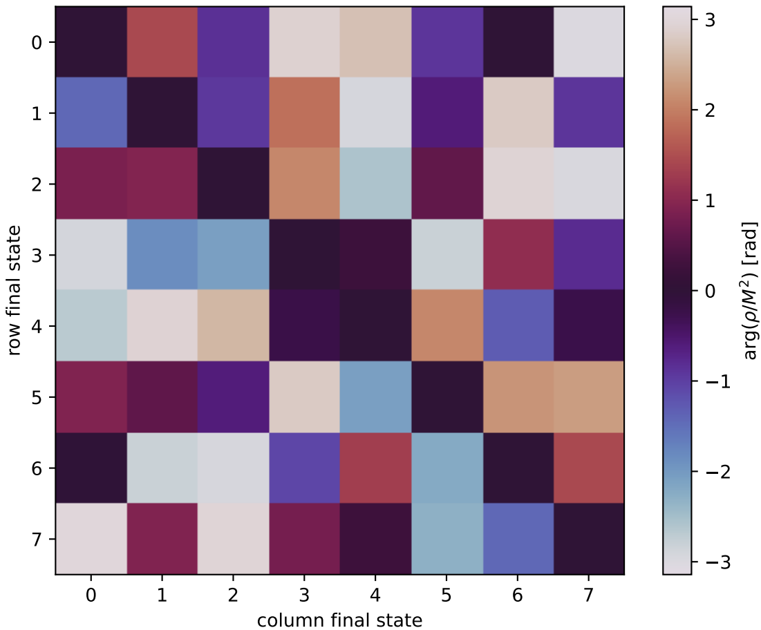
\arg(\rho/M^2) at unpolarized, Q^2=3.5 , t=-1
