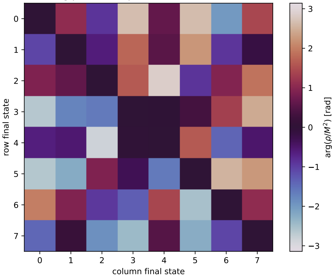
\arg(\rho/M^2) at unpolarized, Q2=4, t=-0.5
