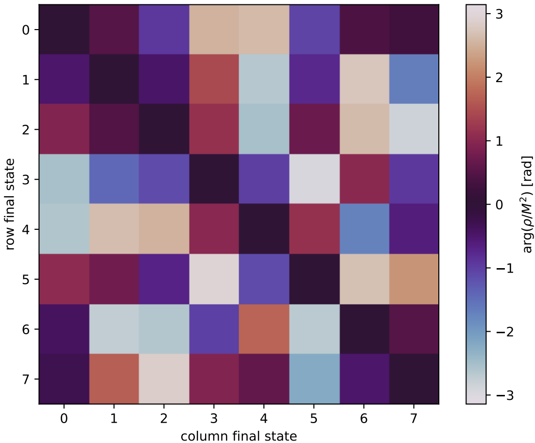
\arg(\rho/M^2) at unpolarized, Q2=5, t=-0.3
