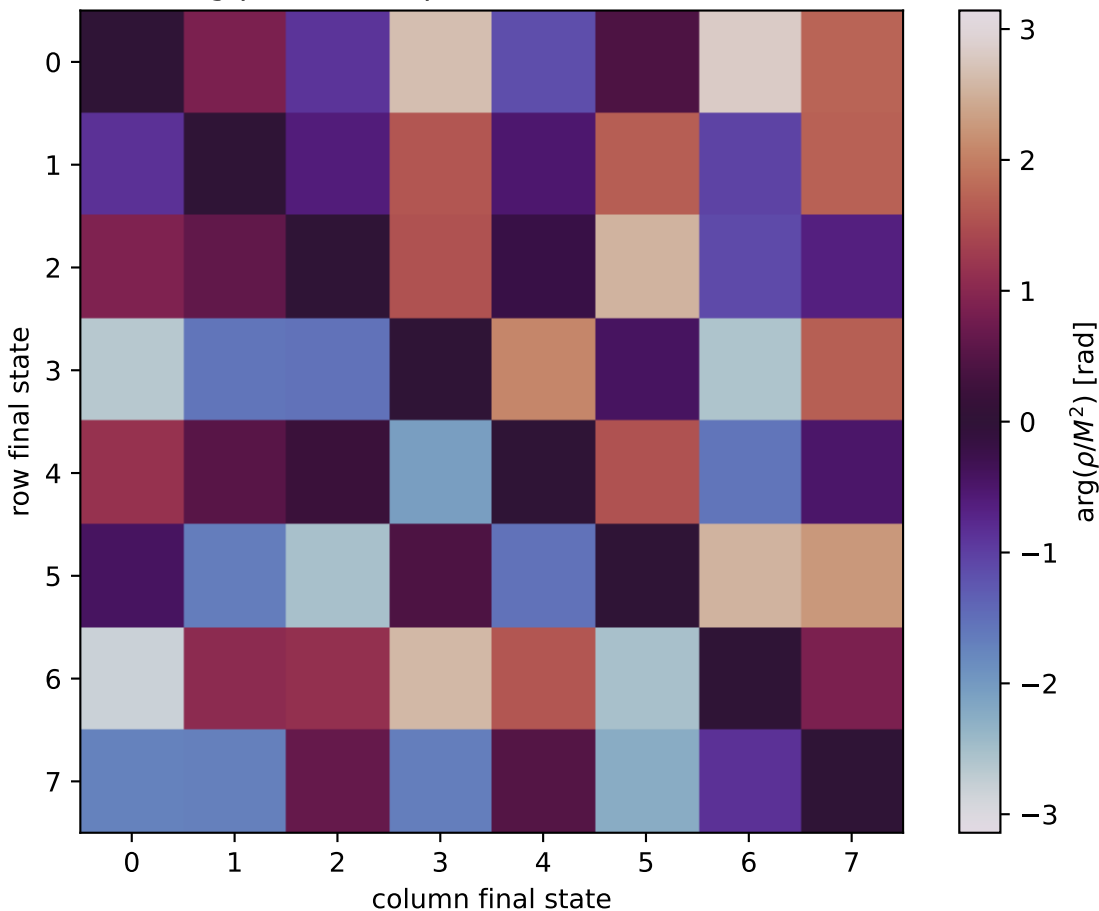
\arg(\rho/M^2) at unpolarized, Q2=5, t=-0.4
