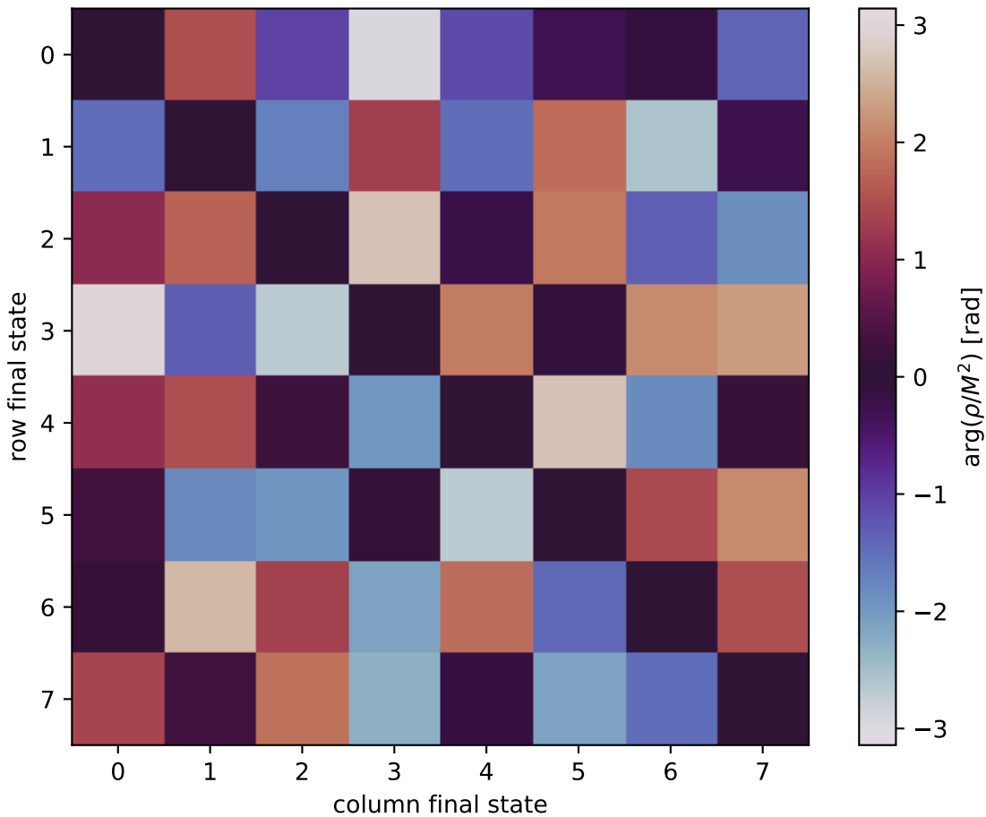
\arg(\rho/M^2) at unpolarized, Q2=6, t=-1.1
