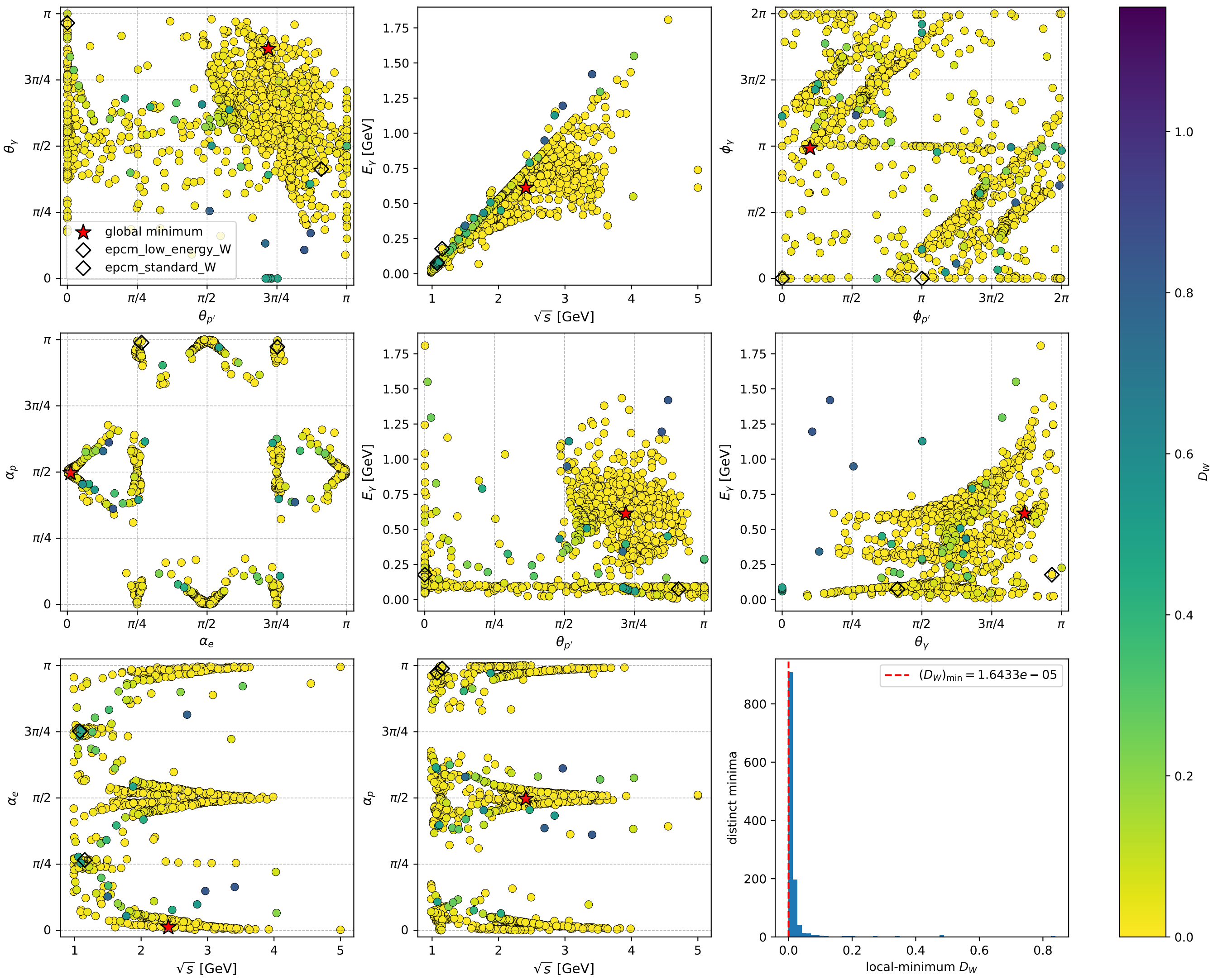
electron: all 1219 distinct gradient-search local minima of D_W
