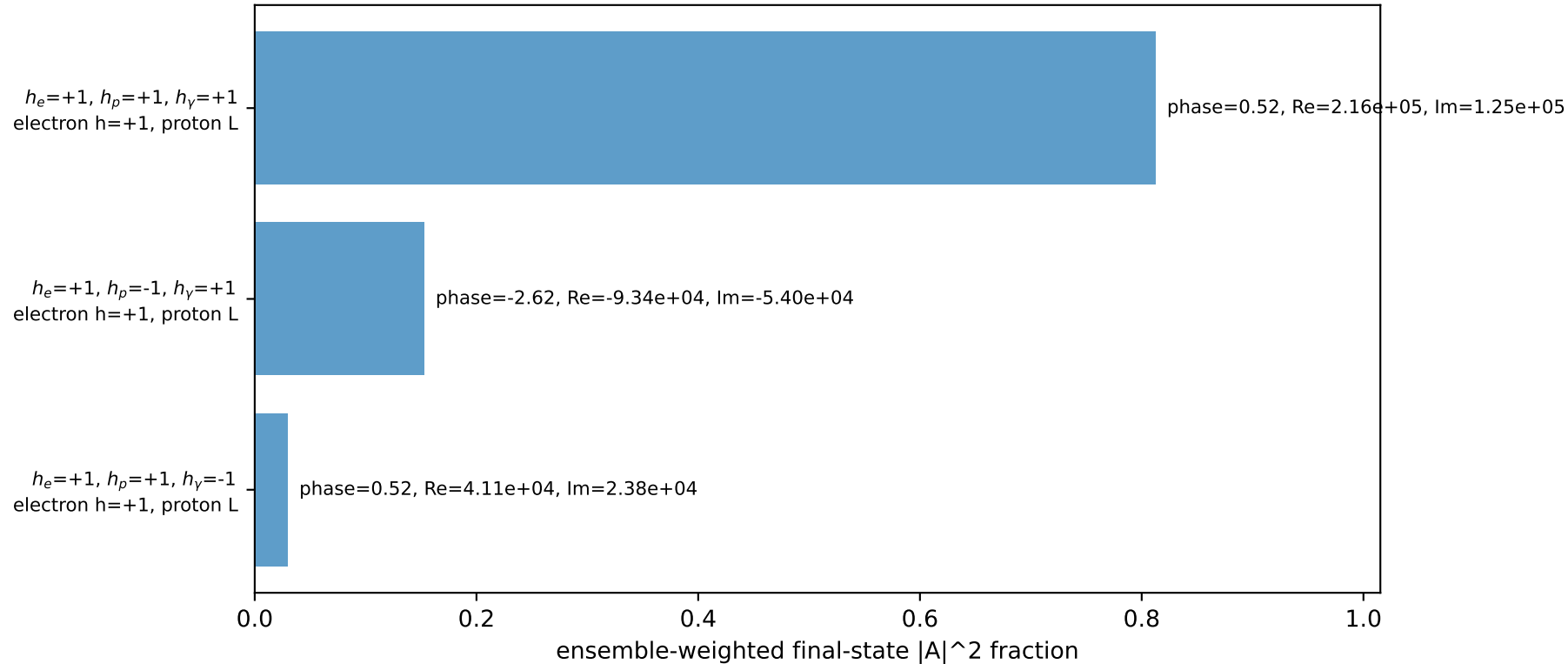
Leading initial-ensemble/final-state components (N=3, retained=99.4%)
