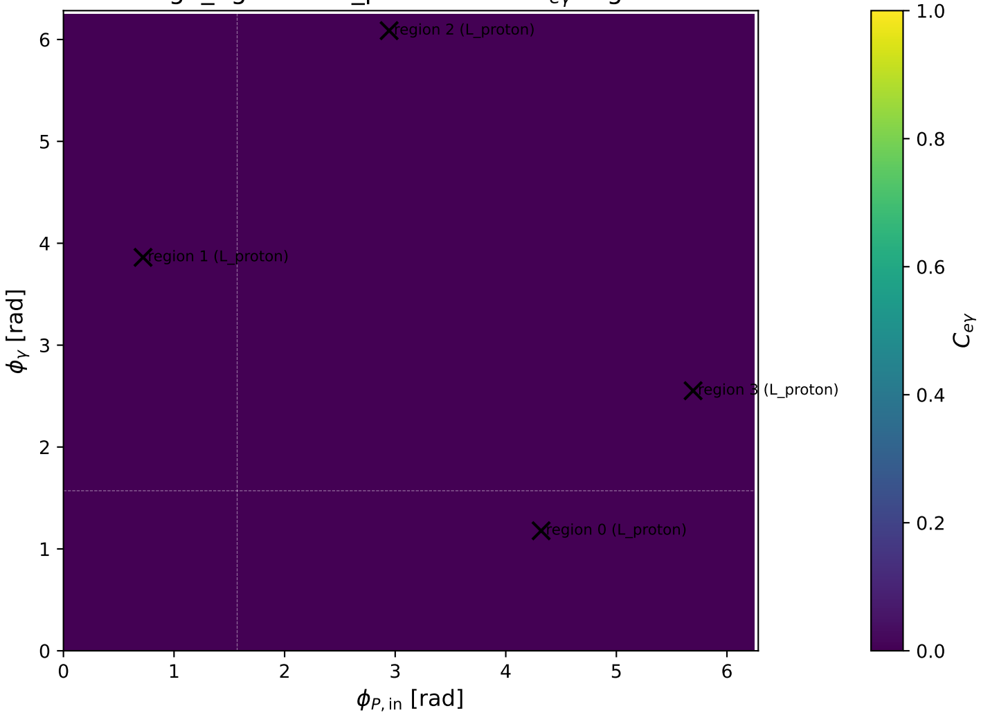
high_Egamma L_proton: max C_{e\gamma} regions
