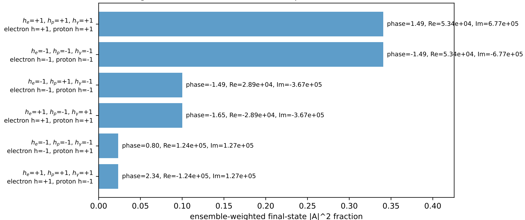
Leading initial-ensemble/final-state components (N=6, retained=92.7%)
