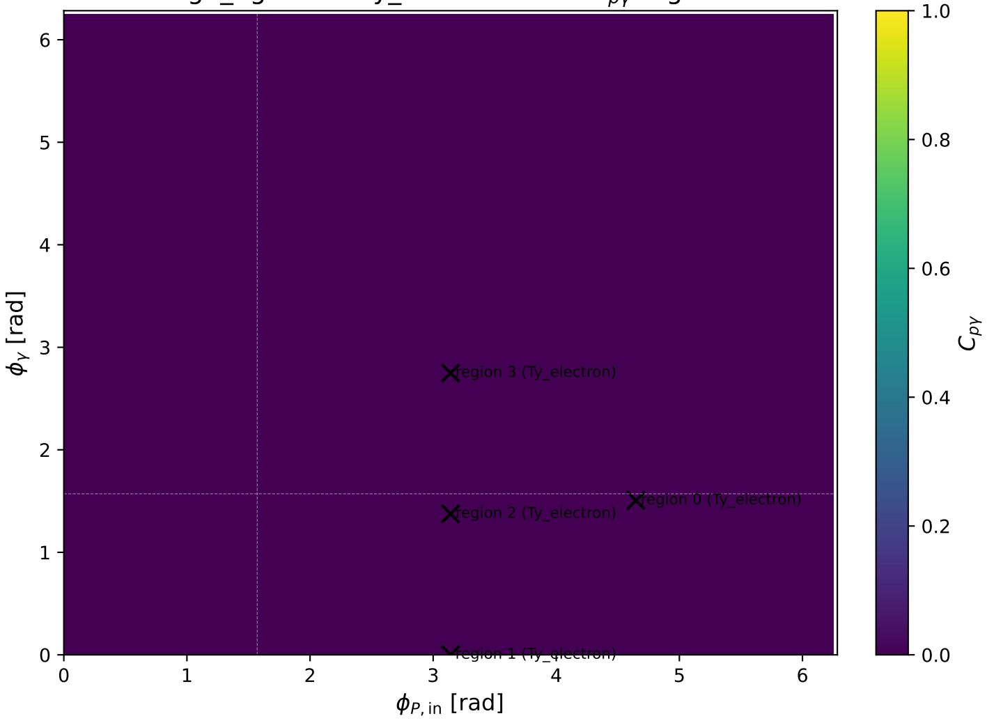
high_Egamma Ty_electron: max C_{p\gamma} regions
