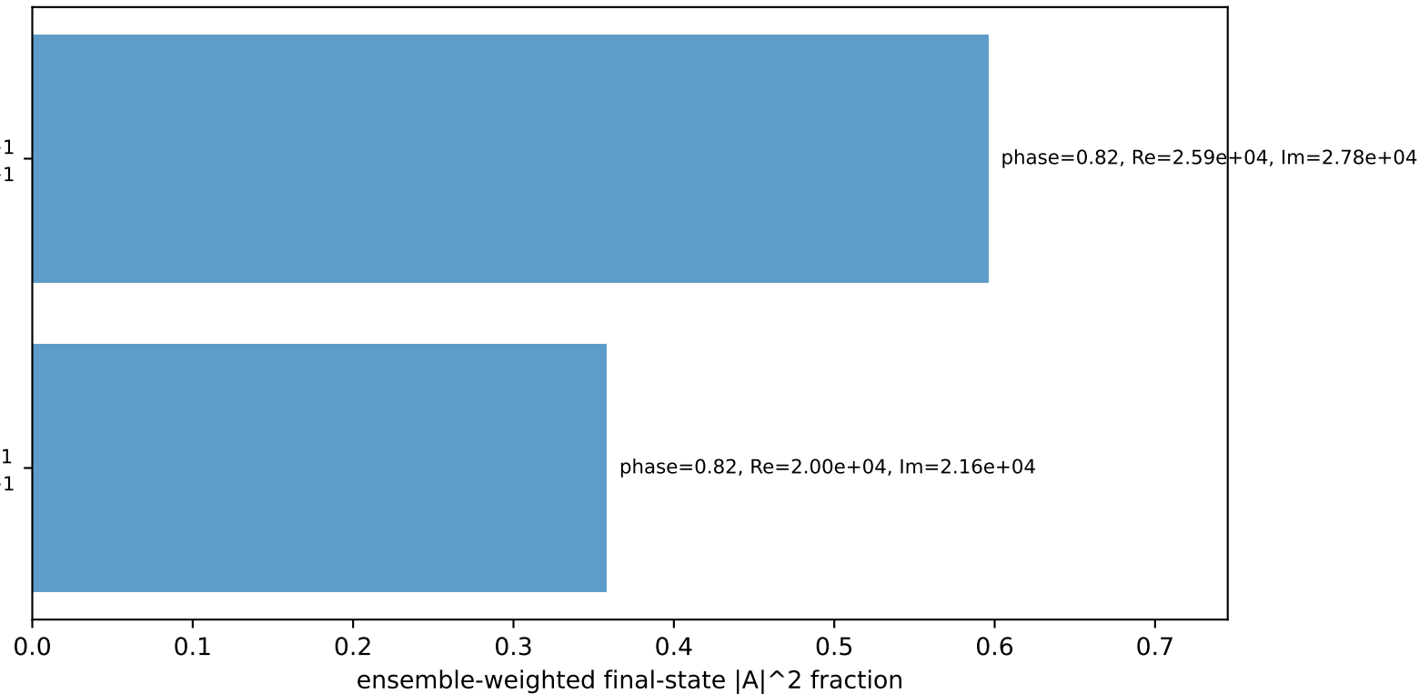
Leading initial-ensemble/final-state components (N=2, retained=95.5%)
