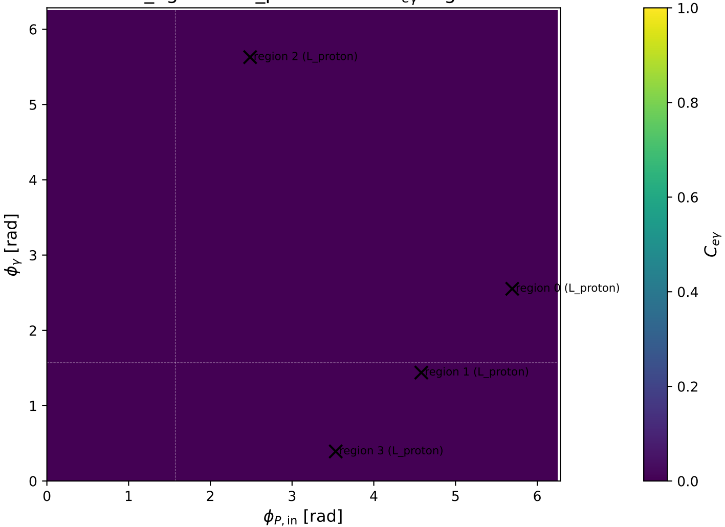
low_Egamma L_proton: max C_{ey} regions
