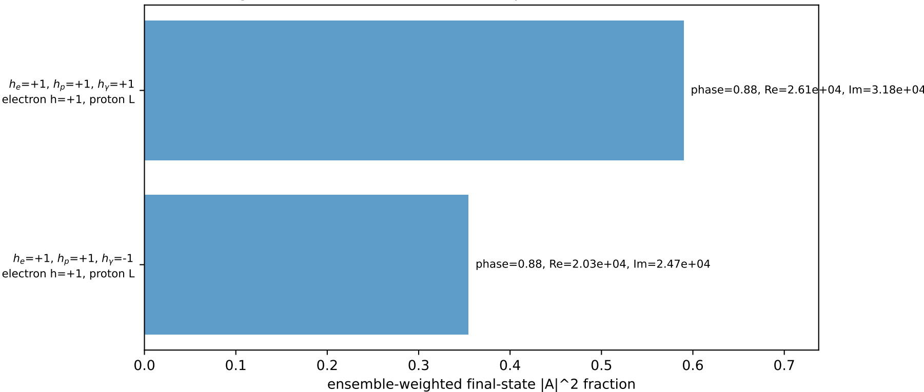
Leading initial-ensemble/final-state components (N=2, retained=94.5%)
