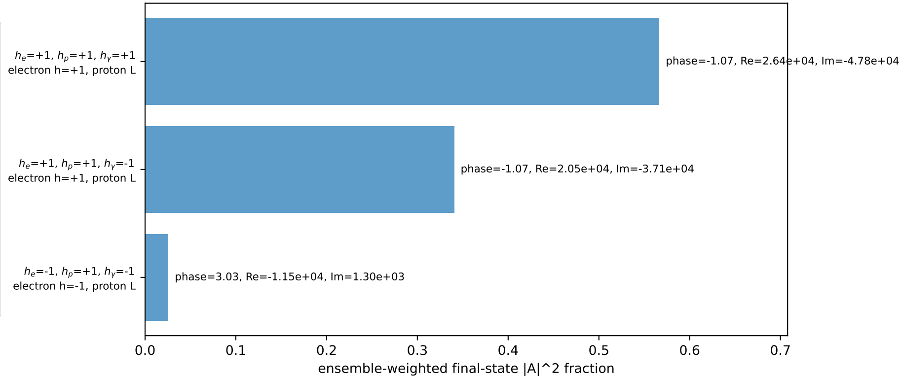
Leading initial-ensemble/final-state components (N=3, retained=93.2%)
