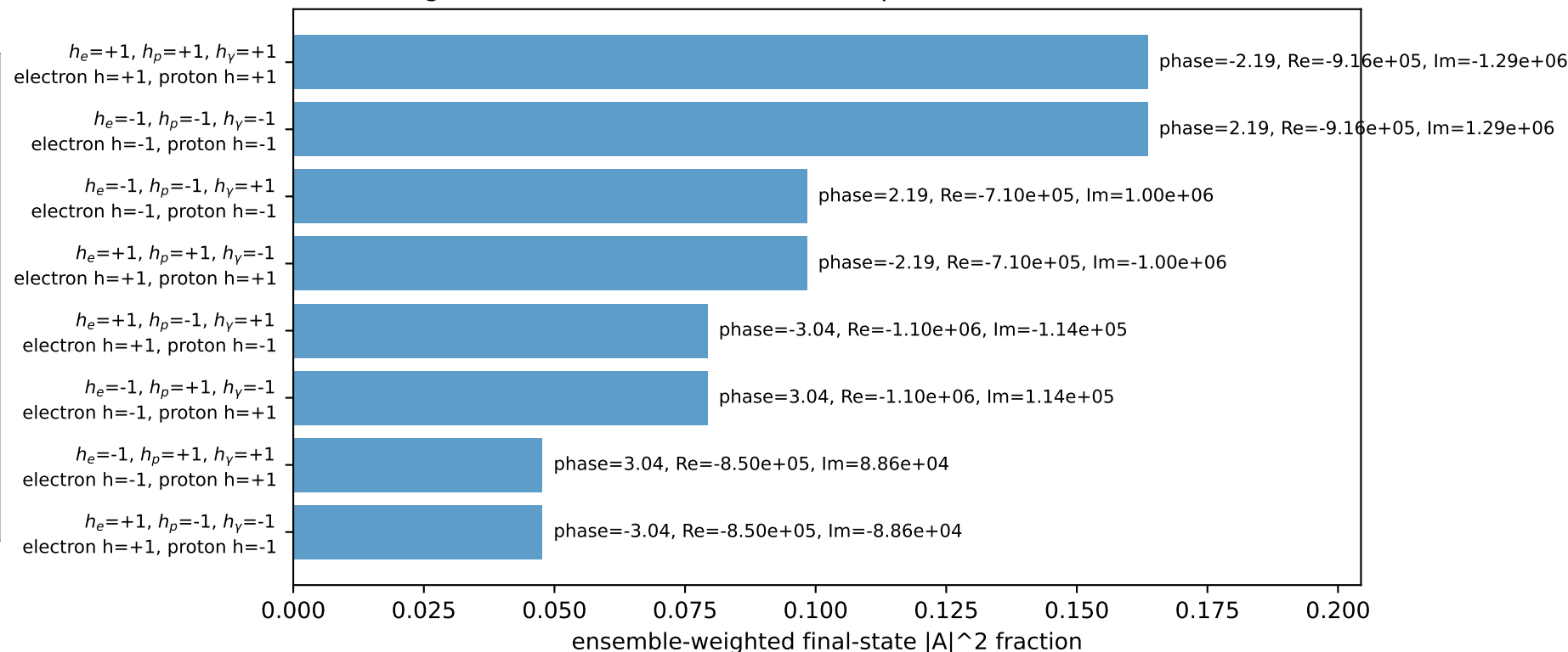
Leading initial-ensemble/final-state components (N=8, retained=77.7%)
