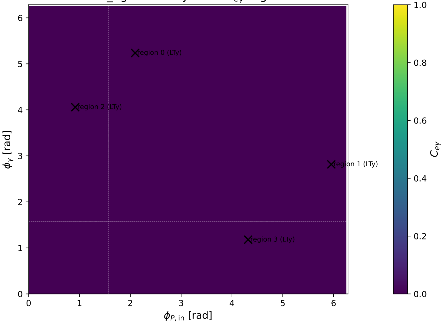
mid_Egamma LTy: max C_{e\gamma} regions
