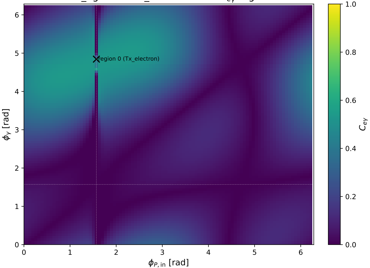
mid_Egamma Tx_electron: max C_{e\gamma} regions
