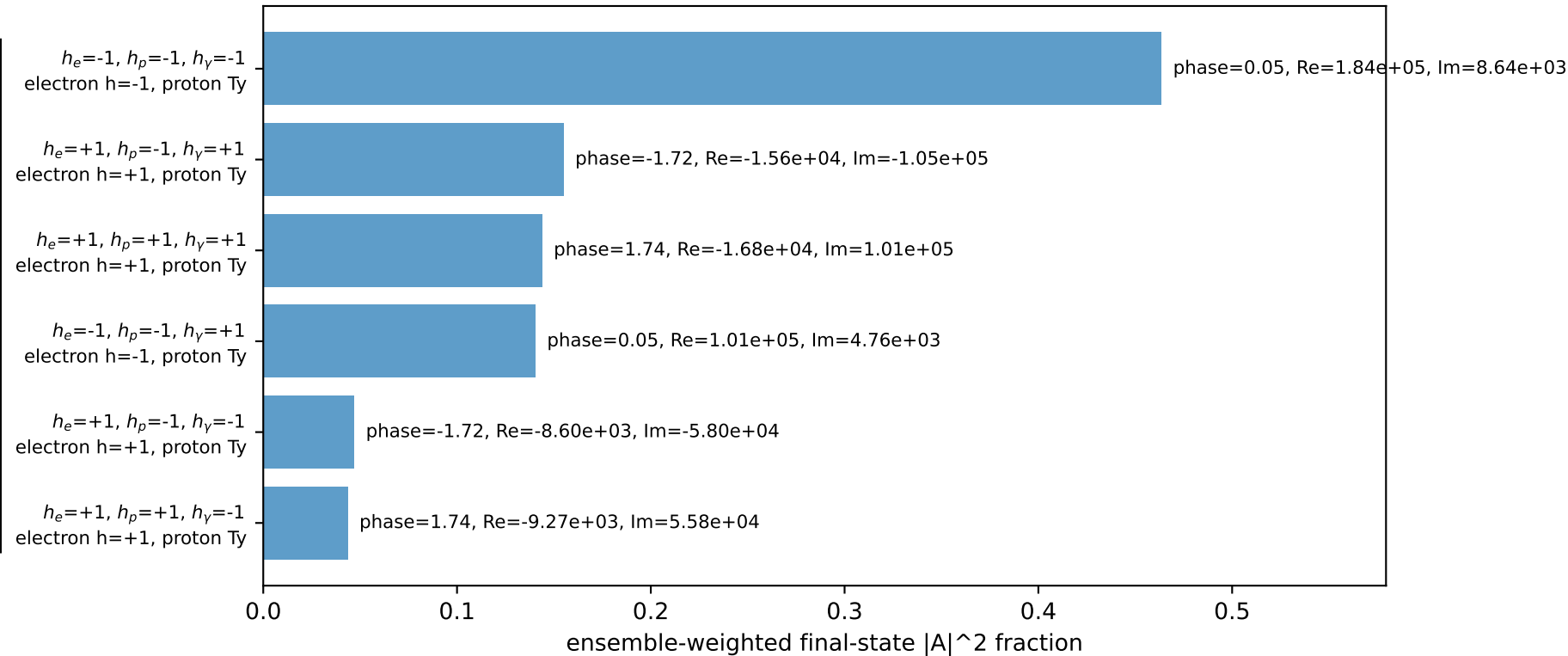
Leading initial-ensemble/final-state components (N=6, retained=99.3%)
