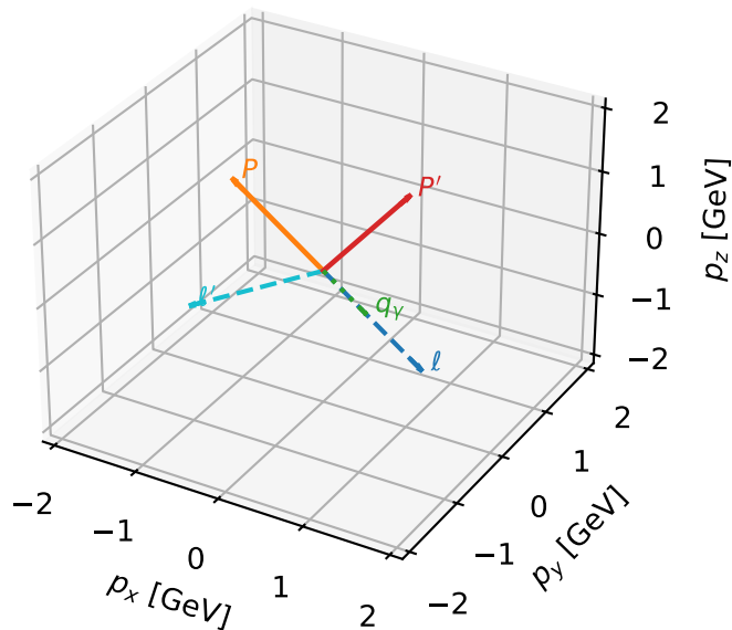
3D momenta
