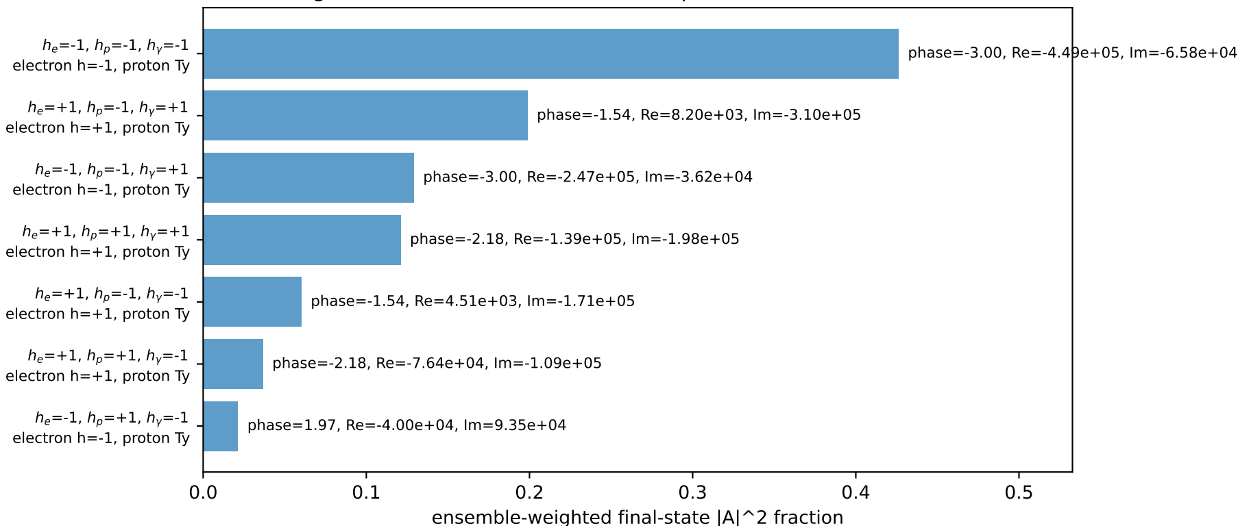
Leading initial-ensemble/final-state components (N=7, retained=99.4%)
