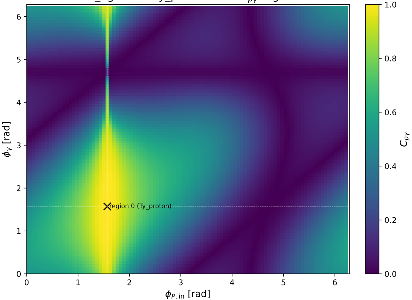
mid_Egamma Ty_proton: max C_{p\gamma} regions
