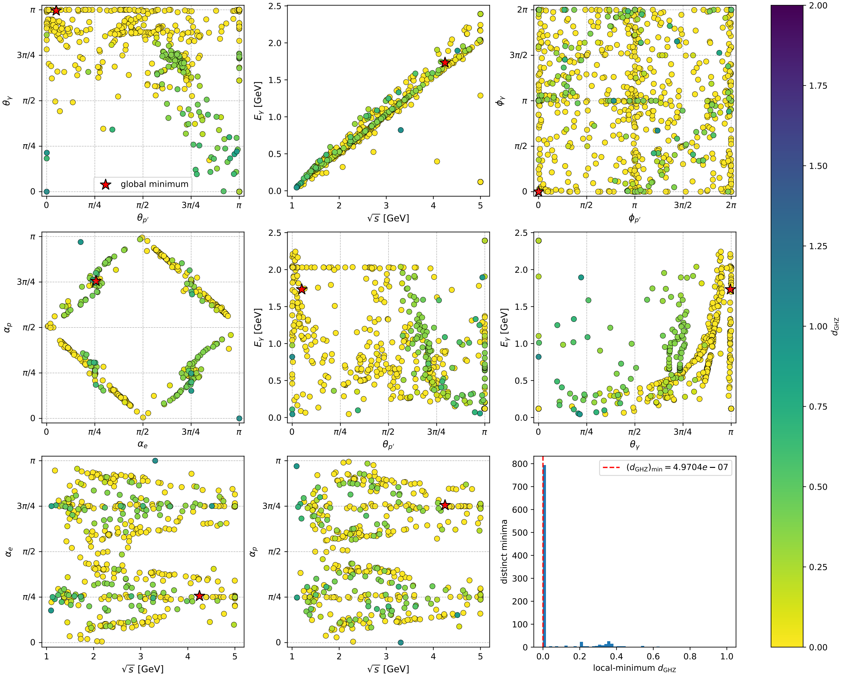
muon: all 953 distinct gradient-search local minima of d_{\text{GHZ}}
