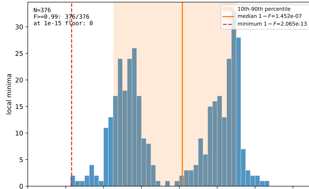
Canonical GHZ LU infidelity (matching target)
