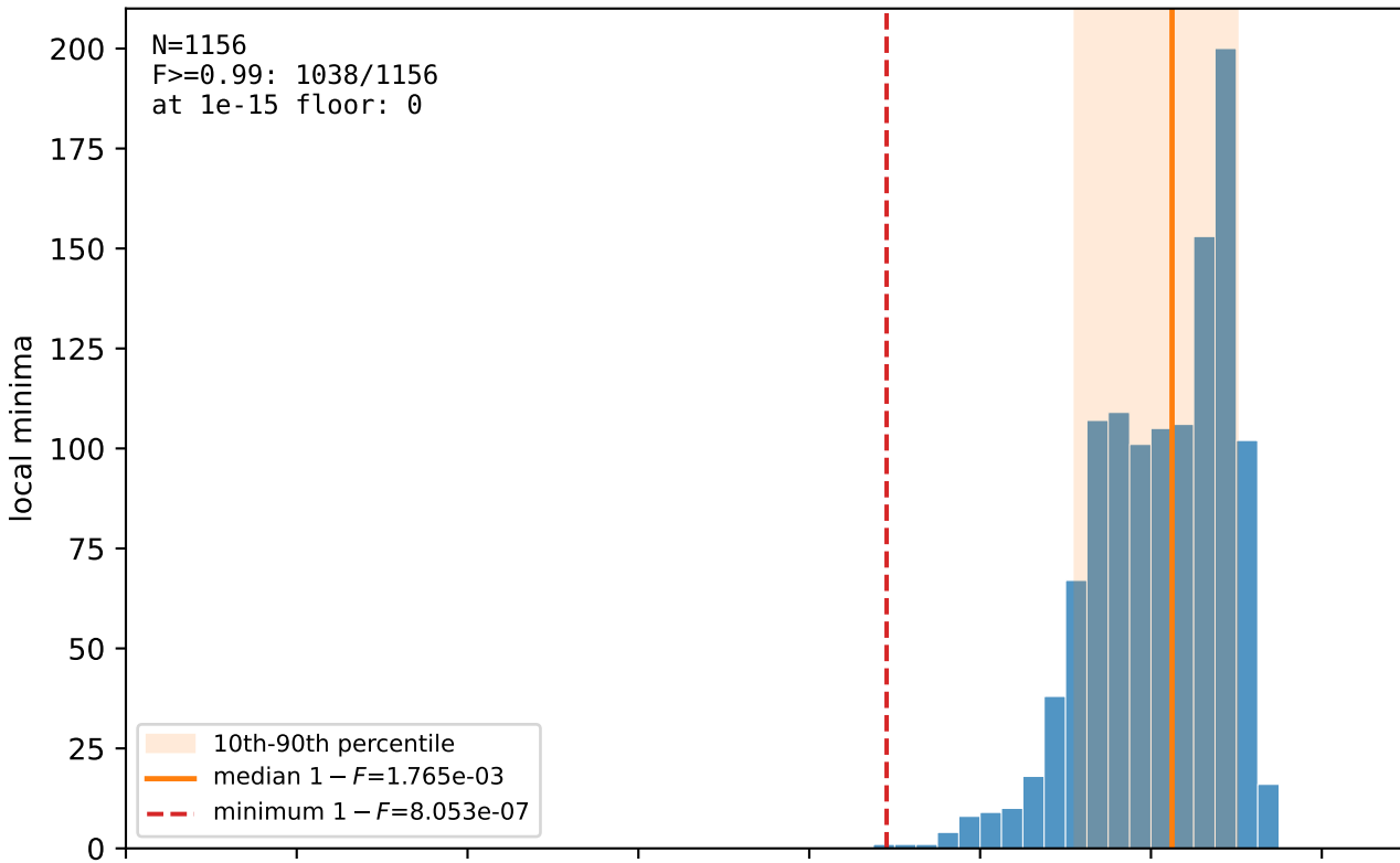
Canonical W LU infidelity (matching target)
