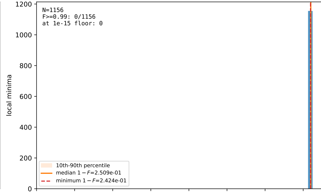
Canonical GHZ LU infidelity
