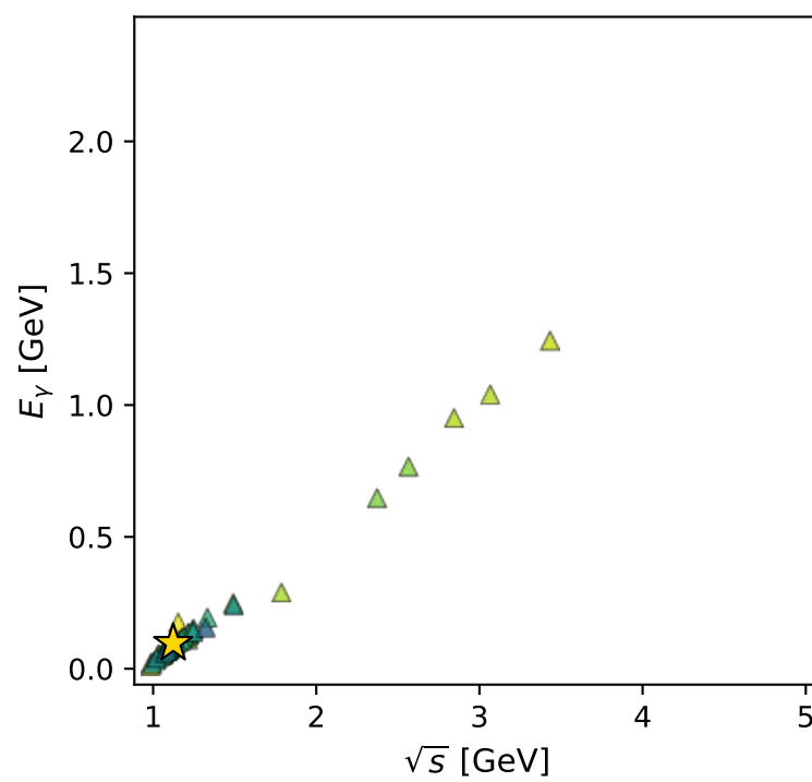
electron: polarization cluster P3; all member minima in phase space
