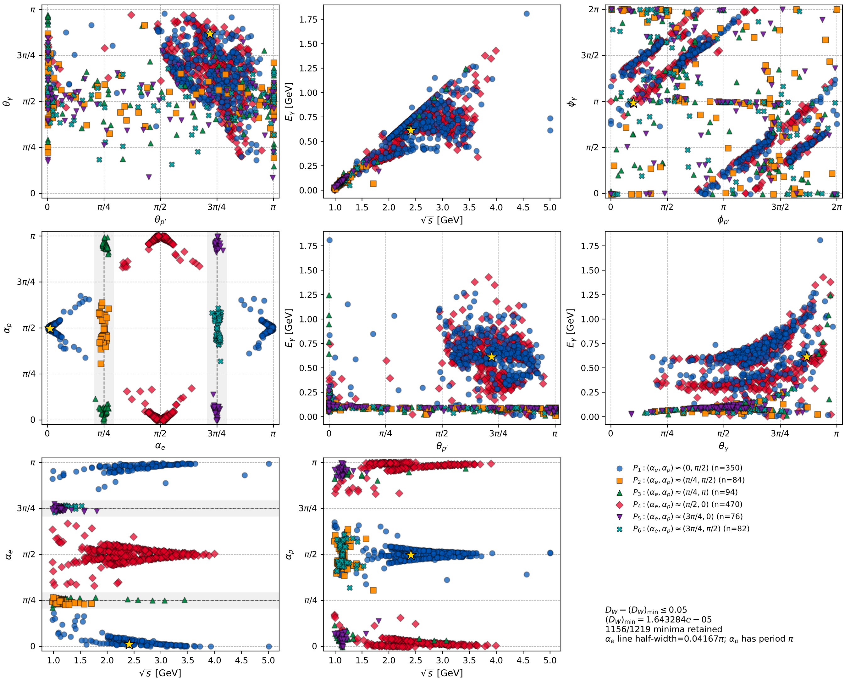
electron: low- D_W phase space colored by 6 major polarization configurations
