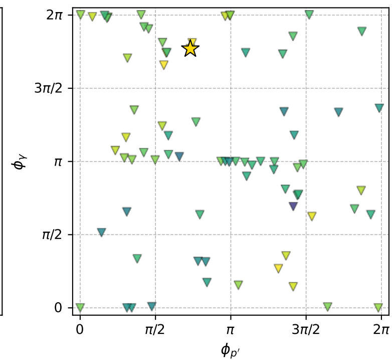
electron: polarization cluster P5; all member minima in phase space
