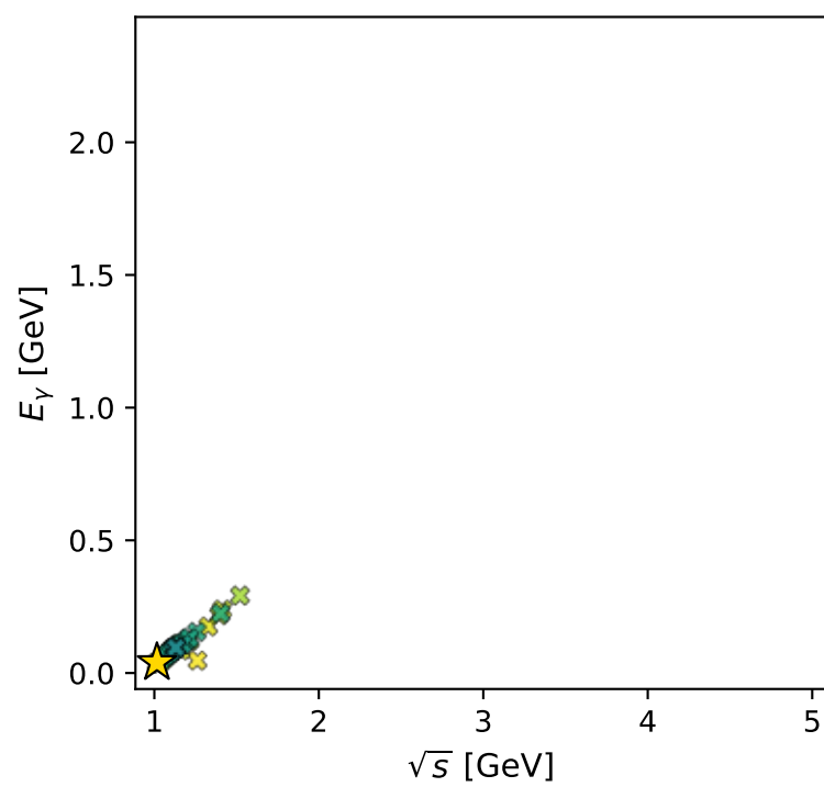
electron: polarization cluster P6; all member minima in phase space
