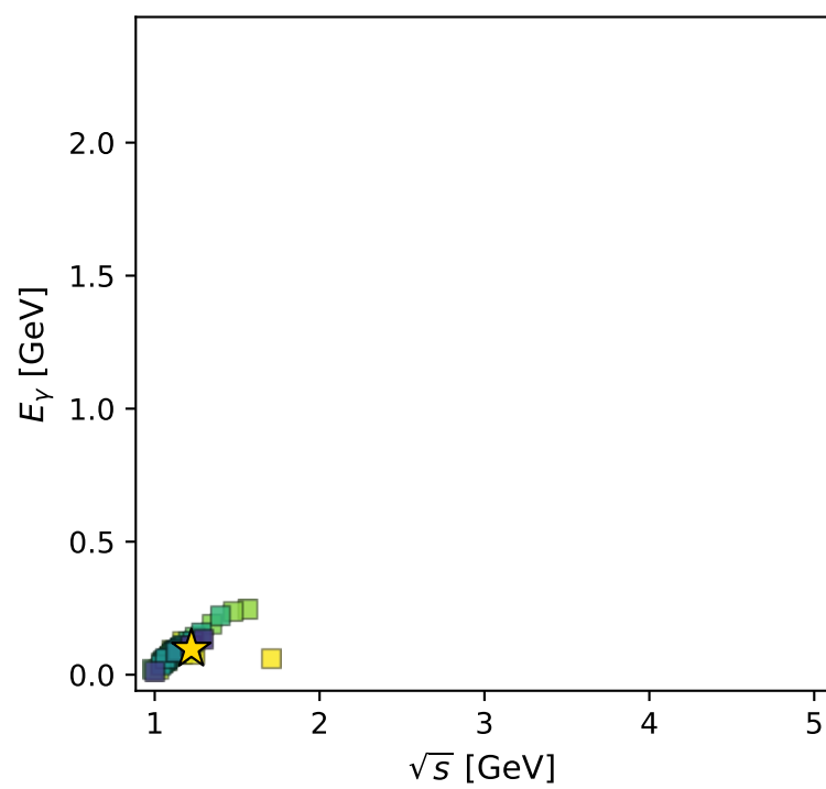
electron: polarization cluster P2; all member minima in phase space
