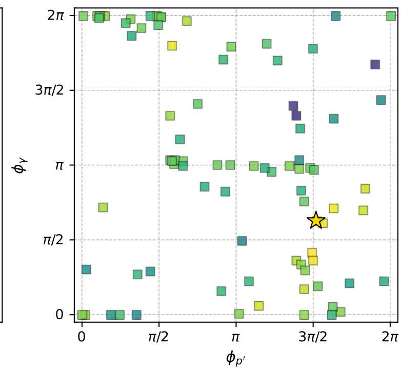
electron: polarization cluster P2; all member minima in phase space
