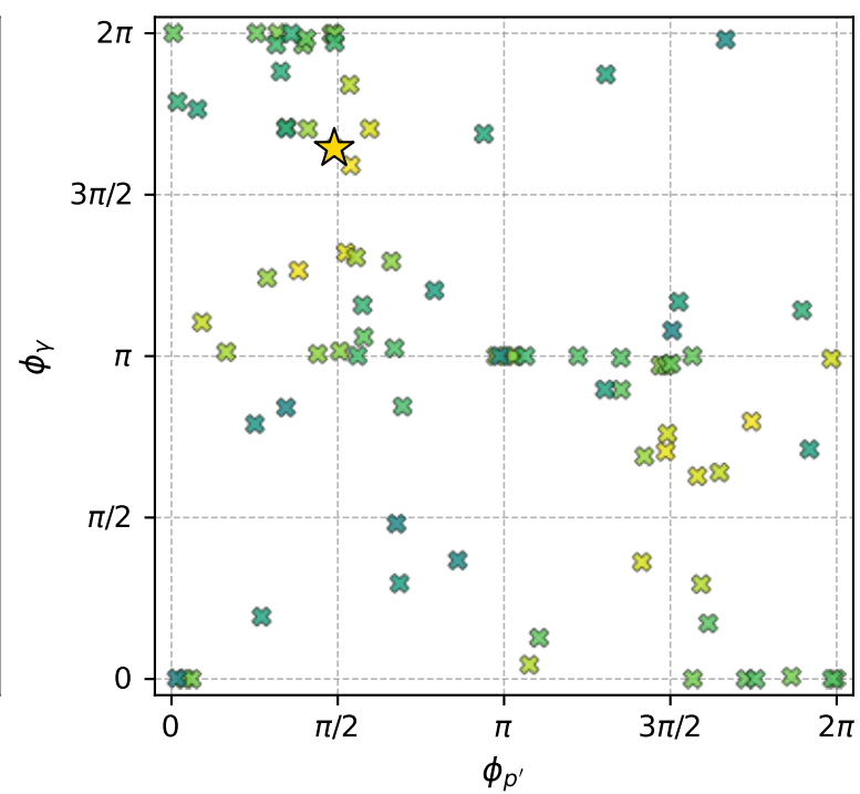
electron: polarization cluster P6; all member minima in phase space
