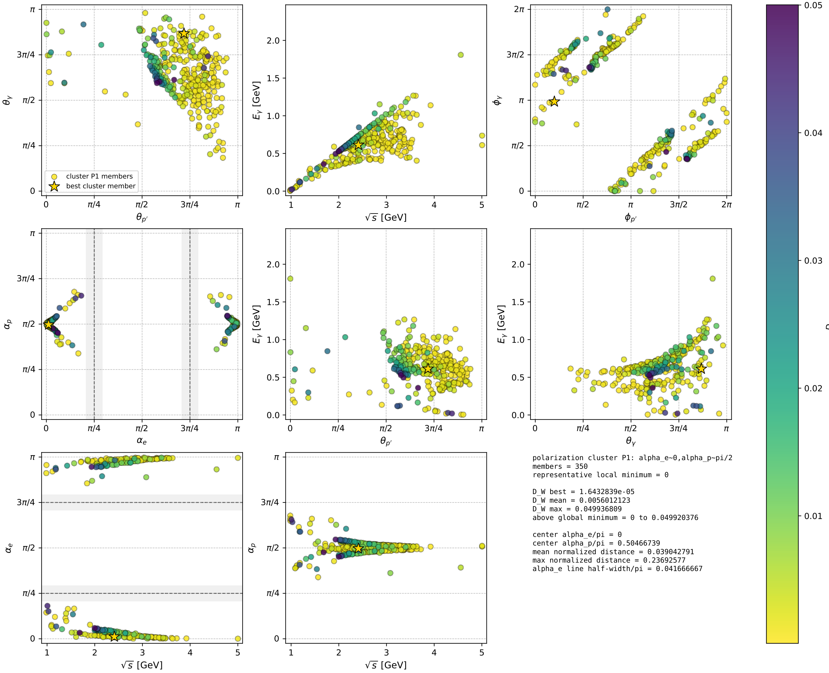
electron: polarization cluster P1; all member minima in phase space
