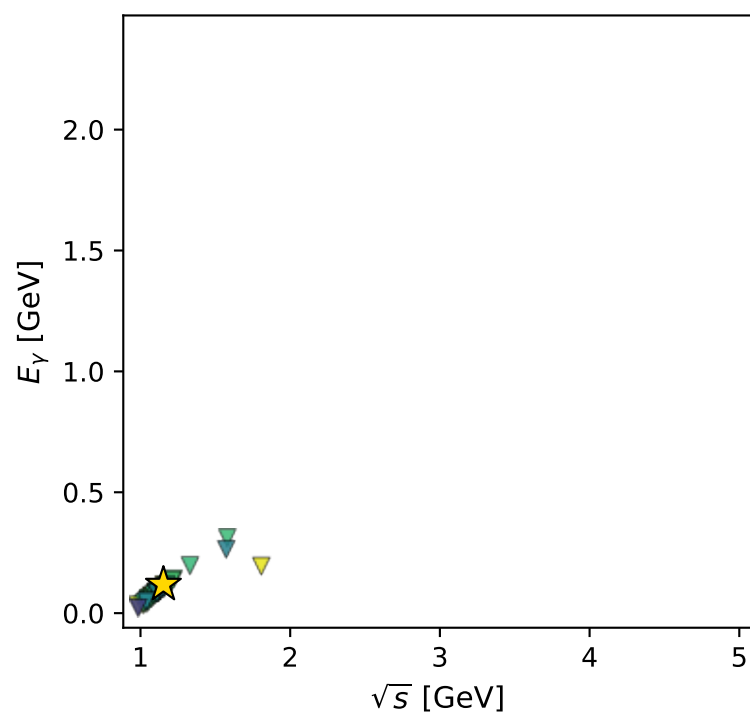
electron: polarization cluster P5; all member minima in phase space
