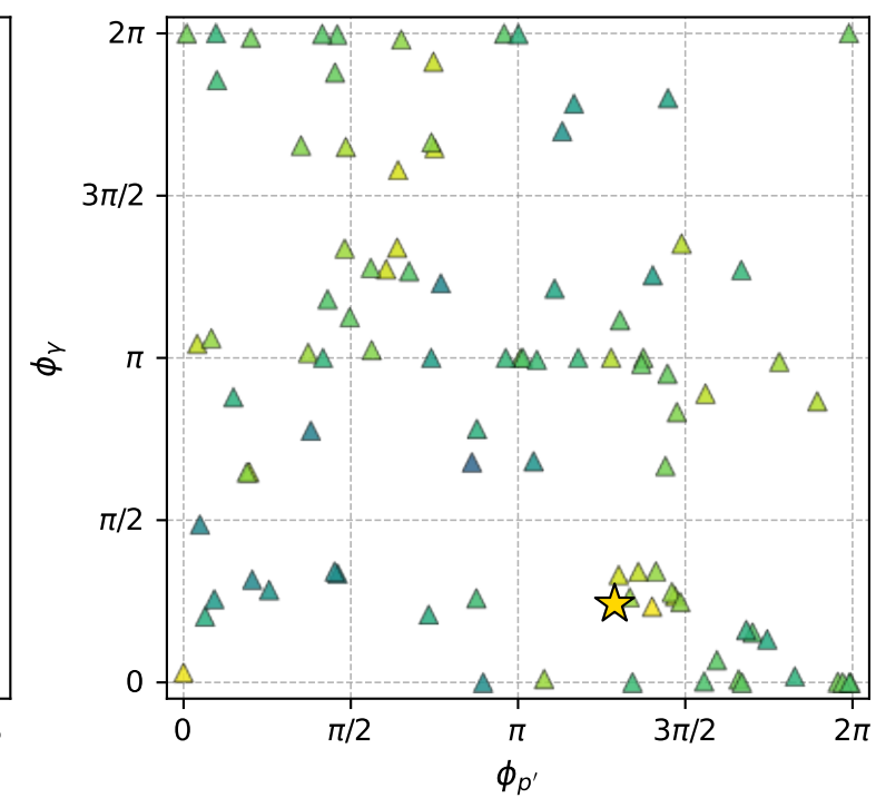
electron: polarization cluster P3; all member minima in phase space
