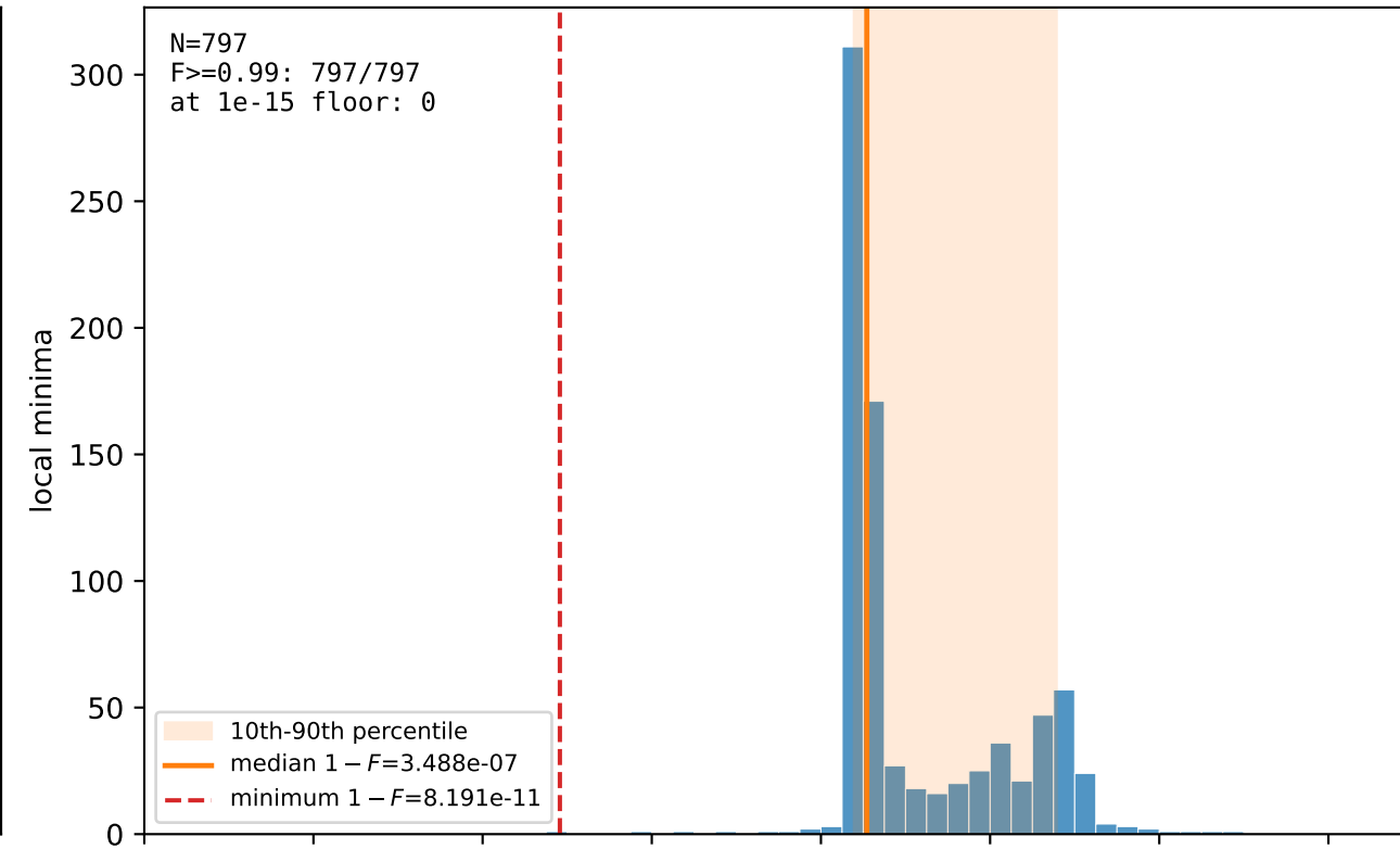
Canonical GHZ LU infidelity (matching target)
