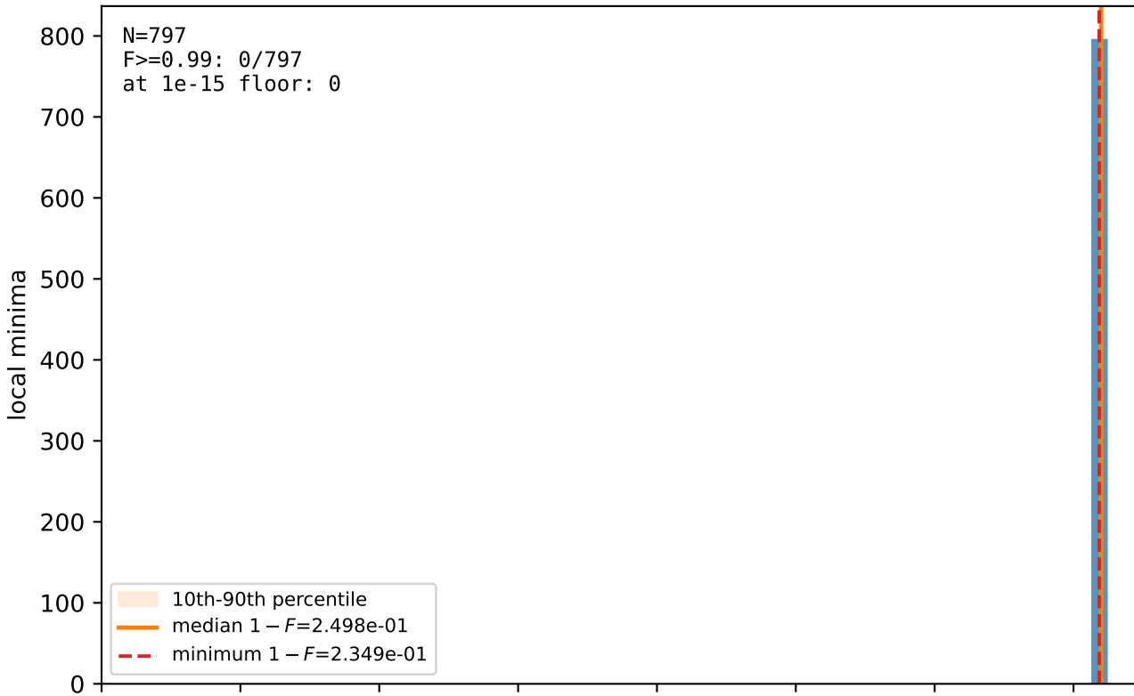
Canonical W LU infidelity
