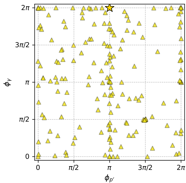
muon: polarization cluster P3; all member minima in phase space
