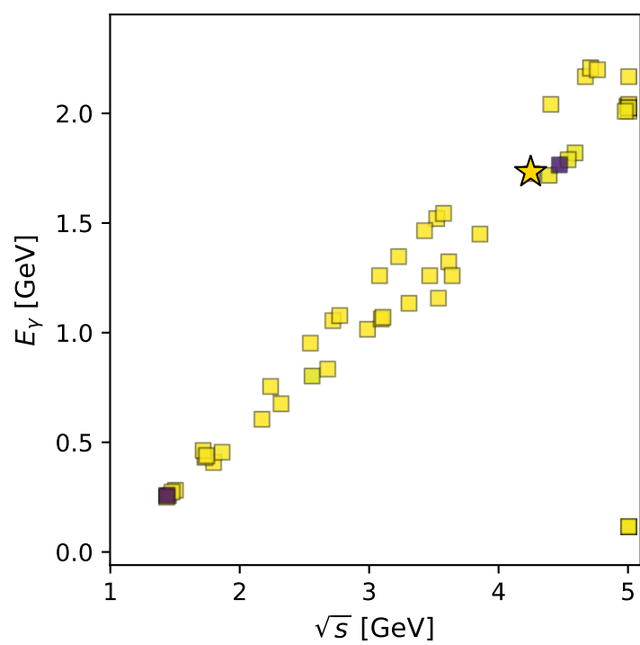
muon: polarization cluster P2; all member minima in phase space
