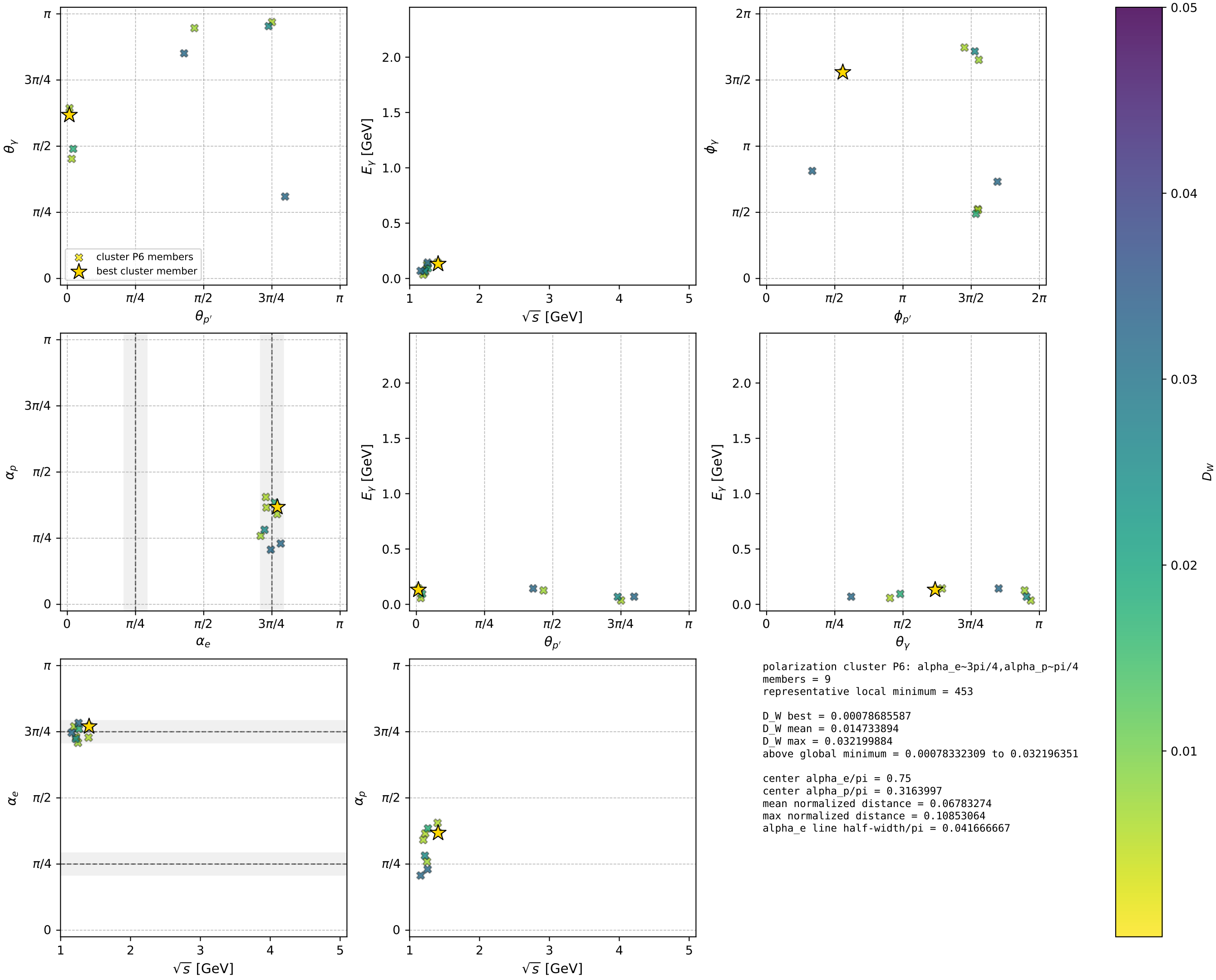
muon: polarization cluster P6; all member minima in phase space
