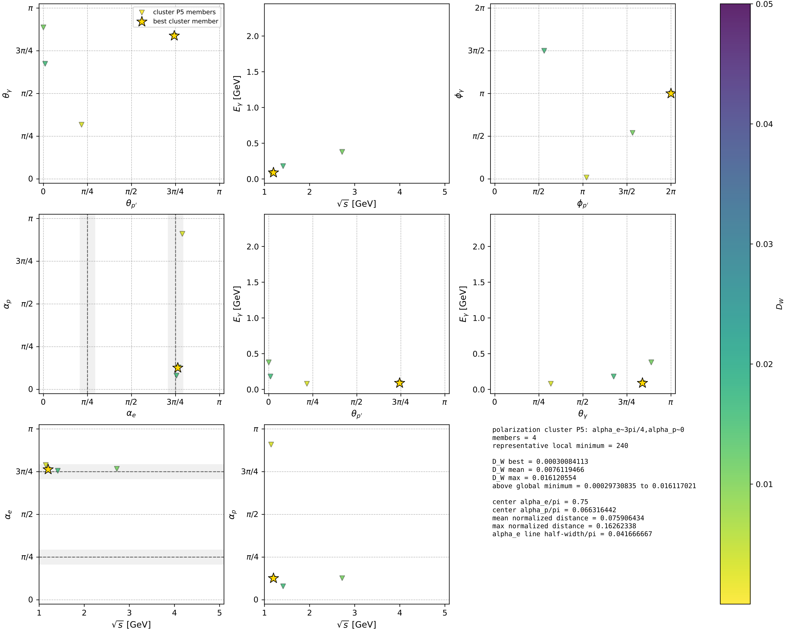
muon: polarization cluster P5; all member minima in phase space
