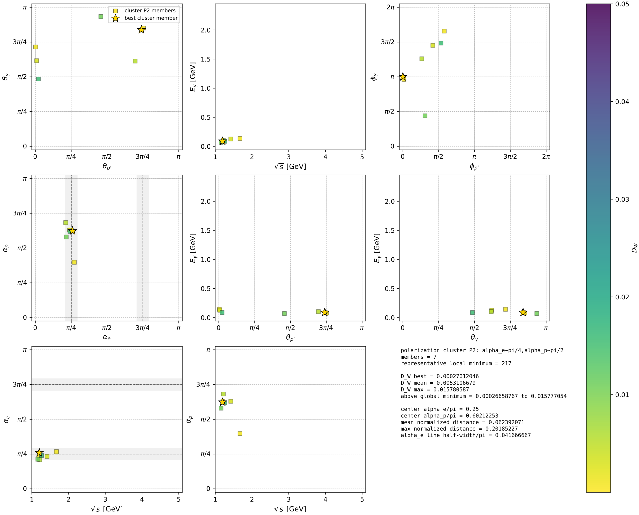
muon: polarization cluster P2; all member minima in phase space
