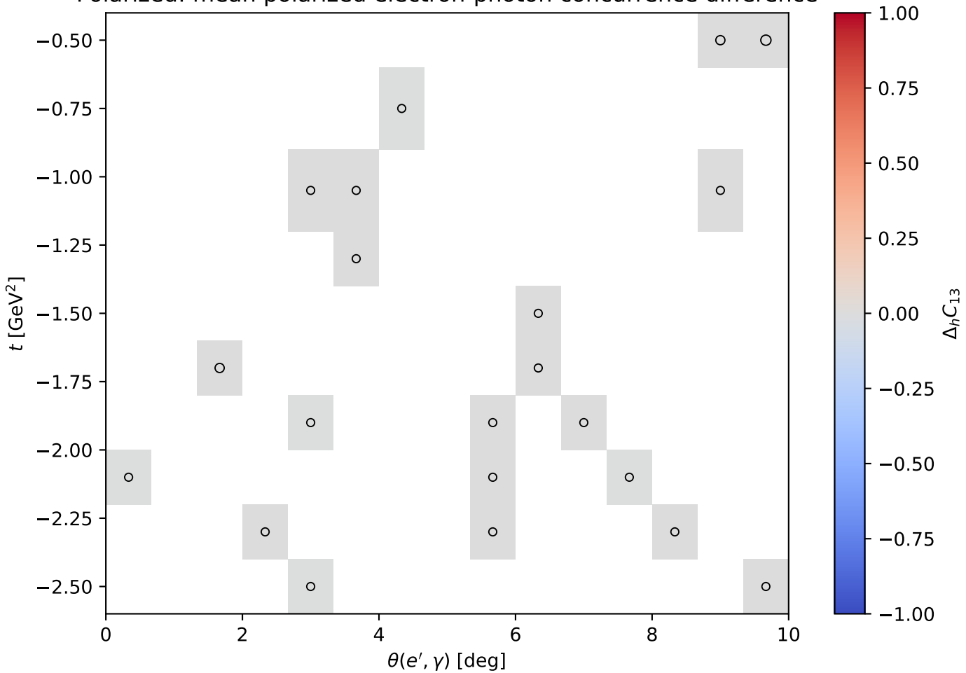
Polarized: mean polarized electron-photon concurrence difference
