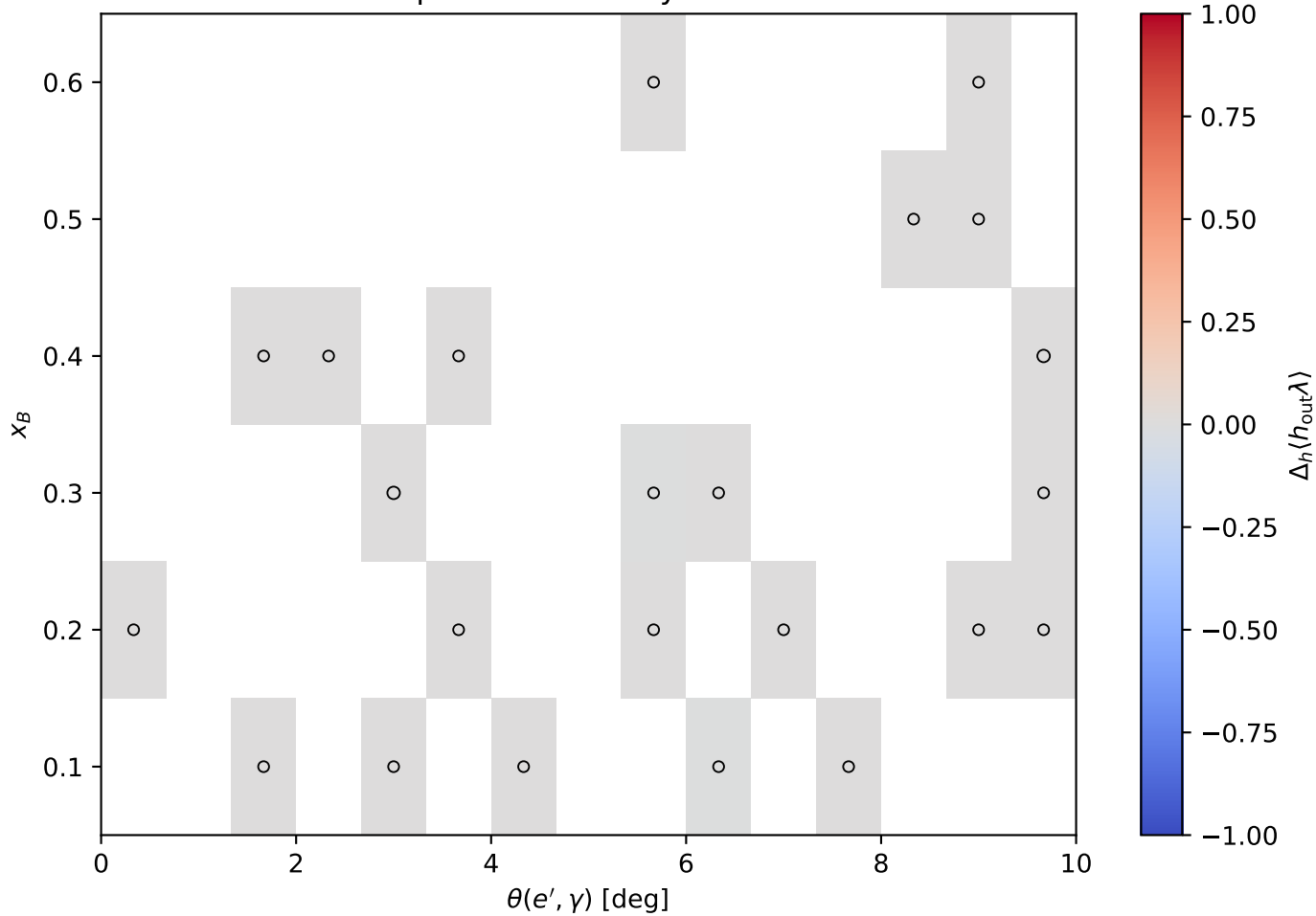
Polarized: mean polarized helicity-difference correlation
