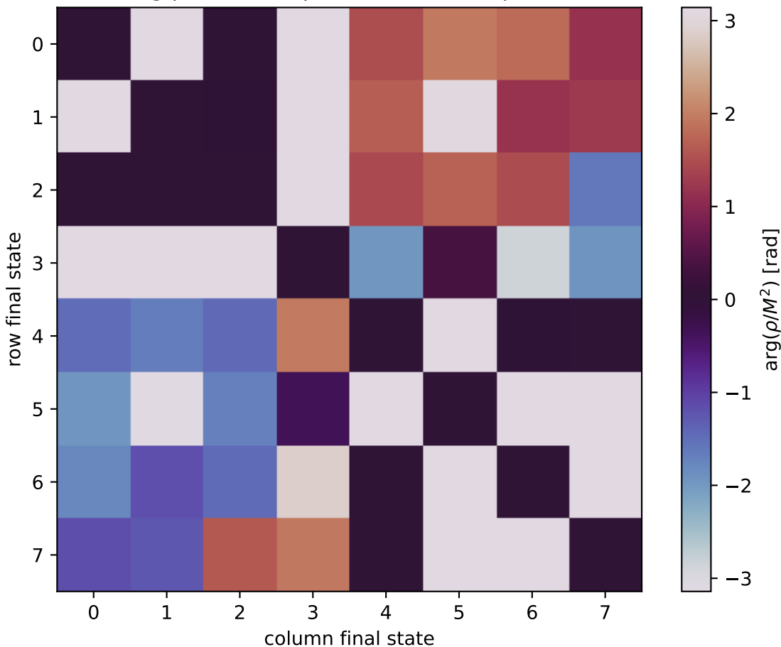
\arg(\rho/M^2) at unpolarized, Q2=3, phi=0
