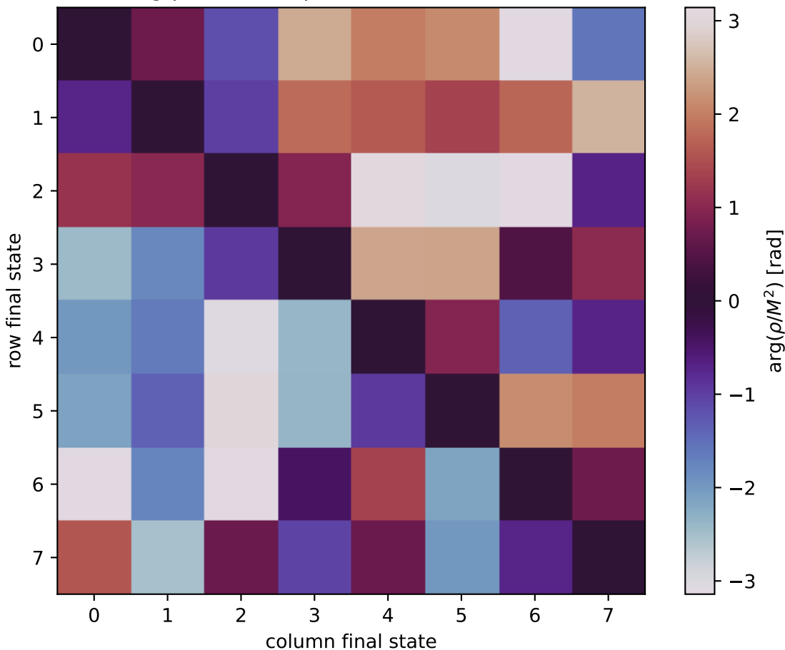
\arg(\rho/M^2) at unpolarized, Q^2=1 , t=-0.8
