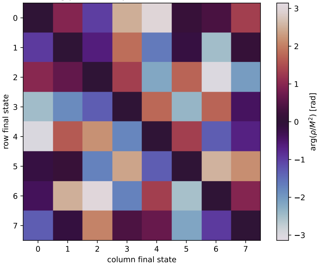
\arg(\rho/M^2) at unpolarized, Q^2=2 , t=-0.6
