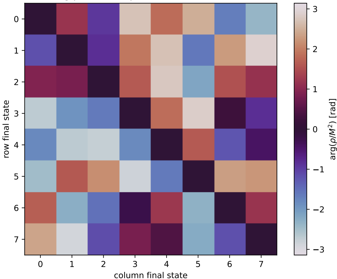
\arg(\rho/M^2) at unpolarized, Q2=2, t=-0.9
