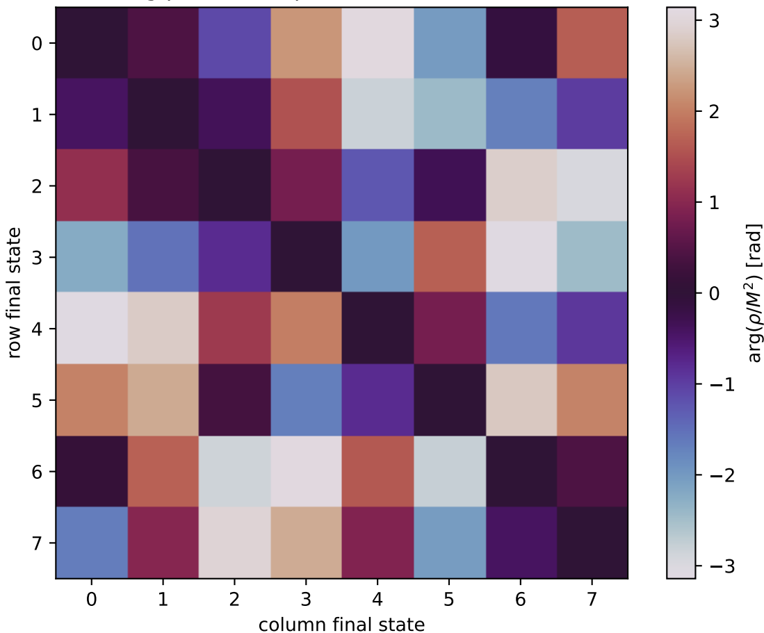
\arg(\rho/M^2) at unpolarized, Q^2=3 , t=-0.3
