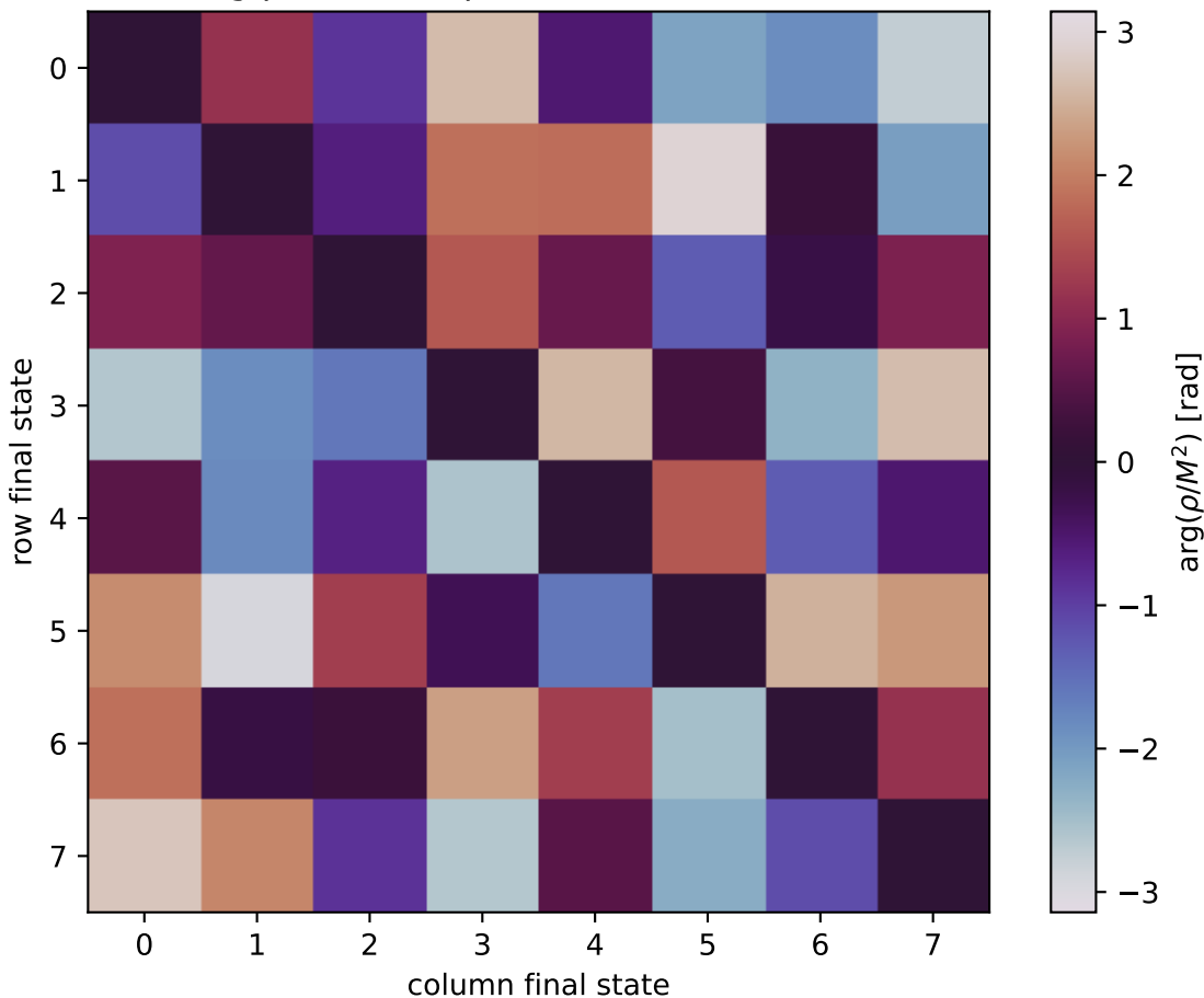
\arg(\rho/M^2) at unpolarized, Q^2=3 , t=-0.6
