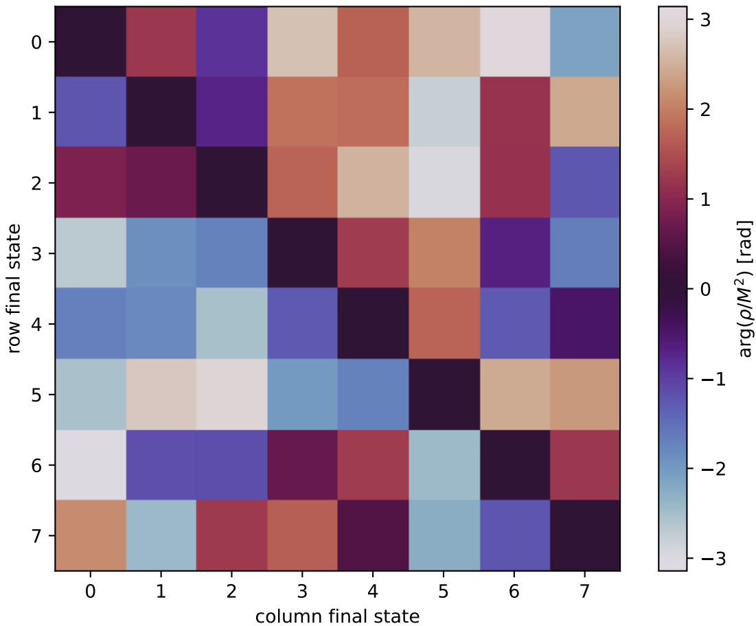
\arg(\rho/M^2) at unpolarized, Q^2=3 , t=-0.7
