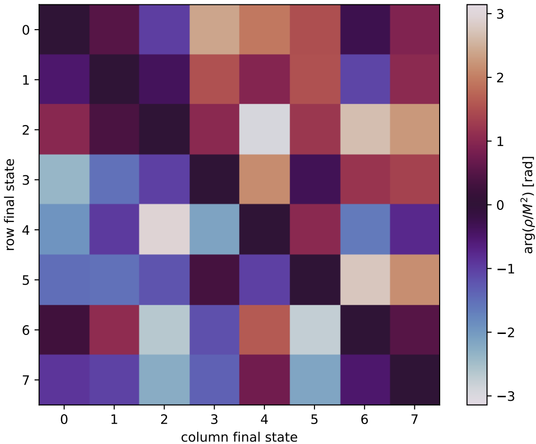
\arg(\rho/M^2) at unpolarized, Q^2=4 , t=-0.3
