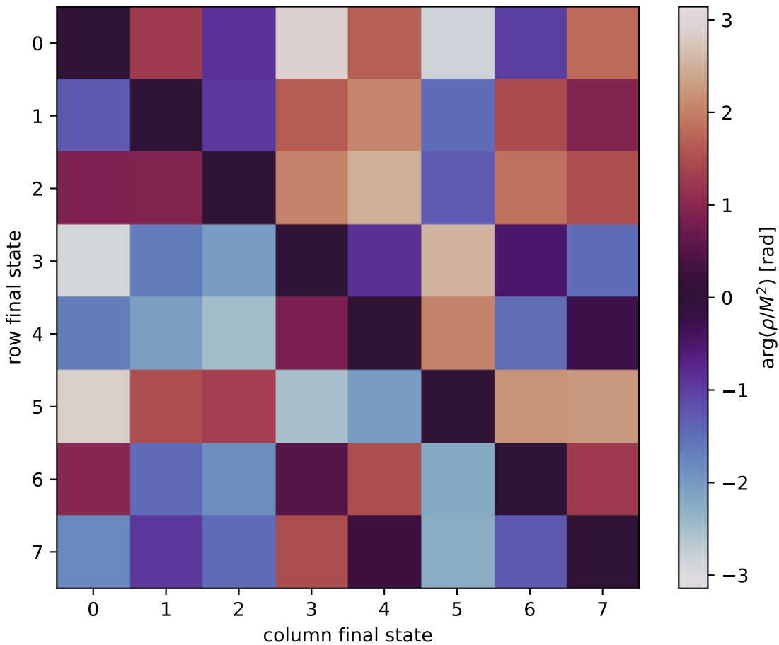
\arg(\rho/M^2) at unpolarized, Q^2=5 , t=-0.7
