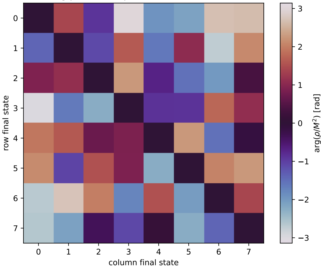
\arg(\rho/M^2) at unpolarized, Q2=5, t=-0.9
