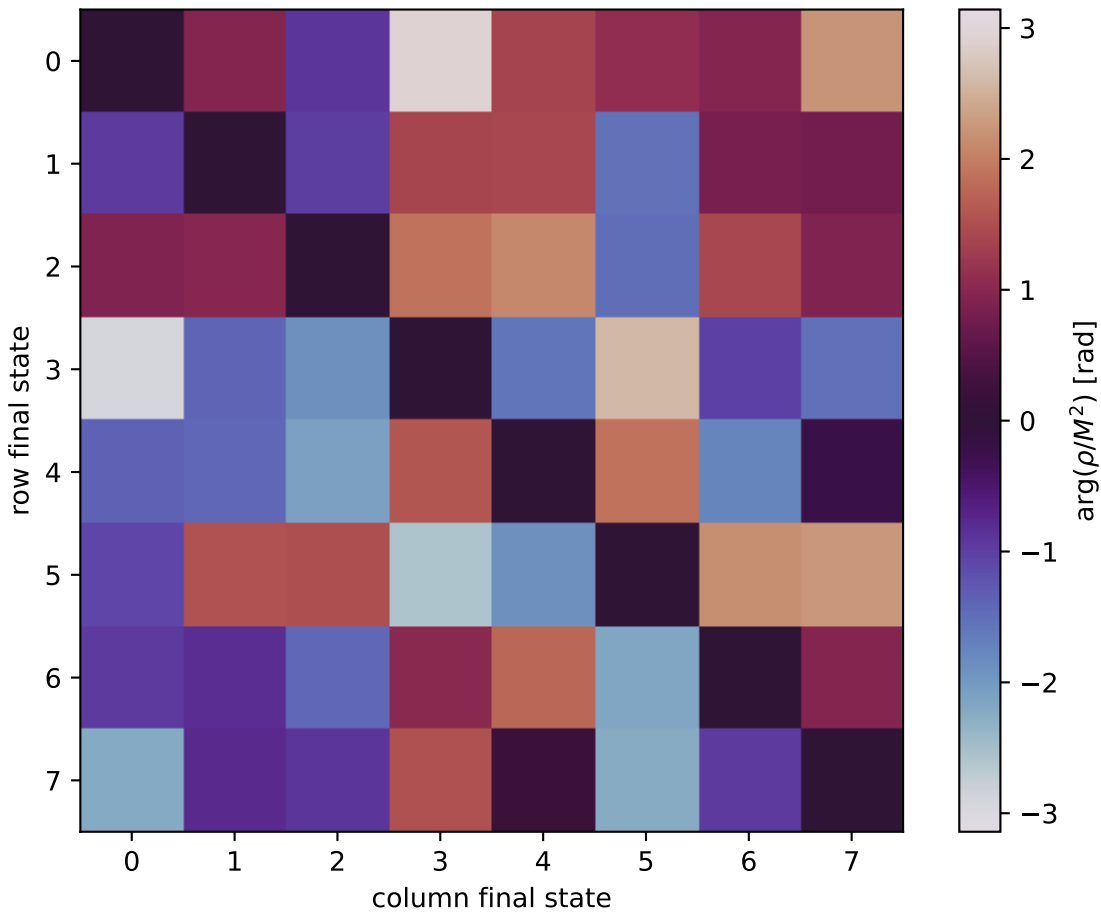
\arg(\rho/M^2) at unpolarized, Q2=6, t=-0.5
