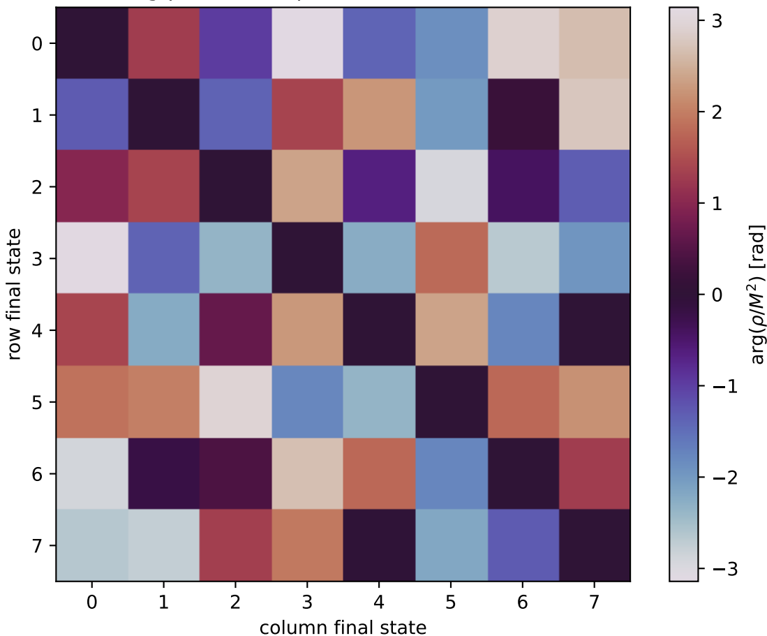
\arg(\rho/M^2) at unpolarized, Q2=6, t=-0.8
