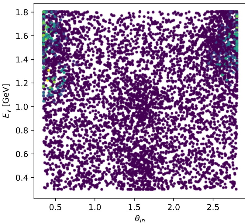
Expanded W search: Tx electron + Tx proton [TxTx], min D_W=0.39901
