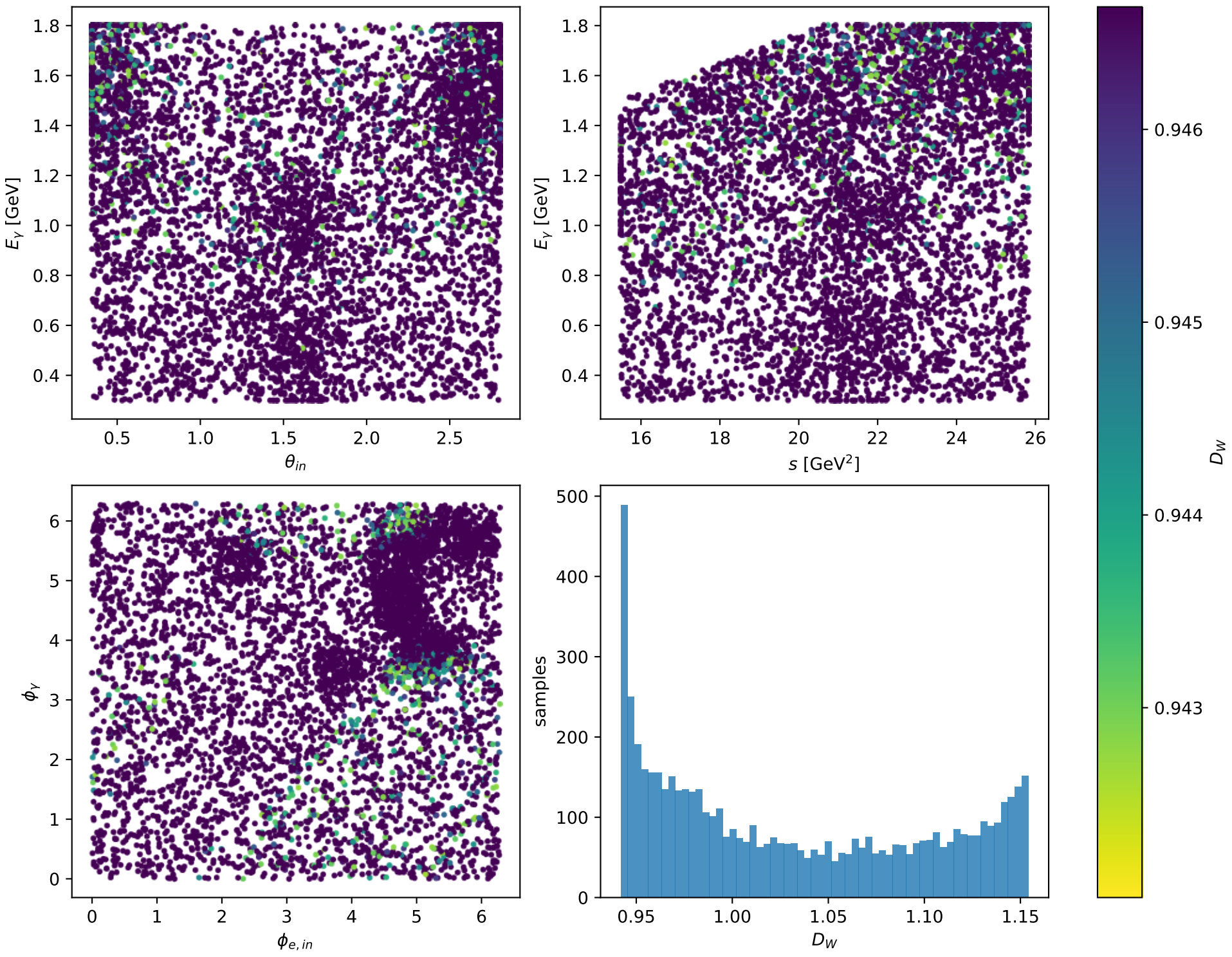
Expanded W search: L electron + Ty proton [LTy], min D_W=0.94202
