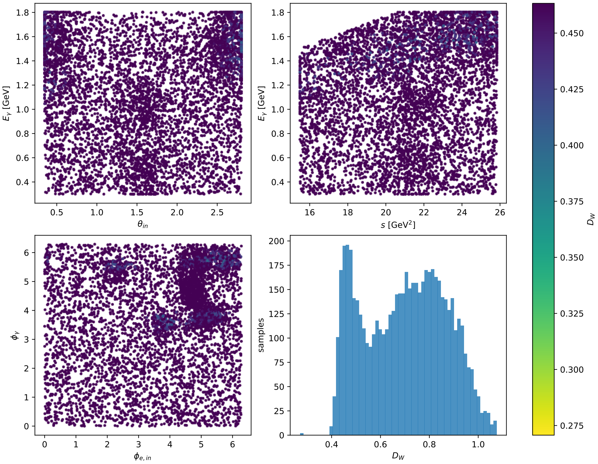
Expanded W search: Tx electron + Ty proton [TxTy], min D_W=0.2707
