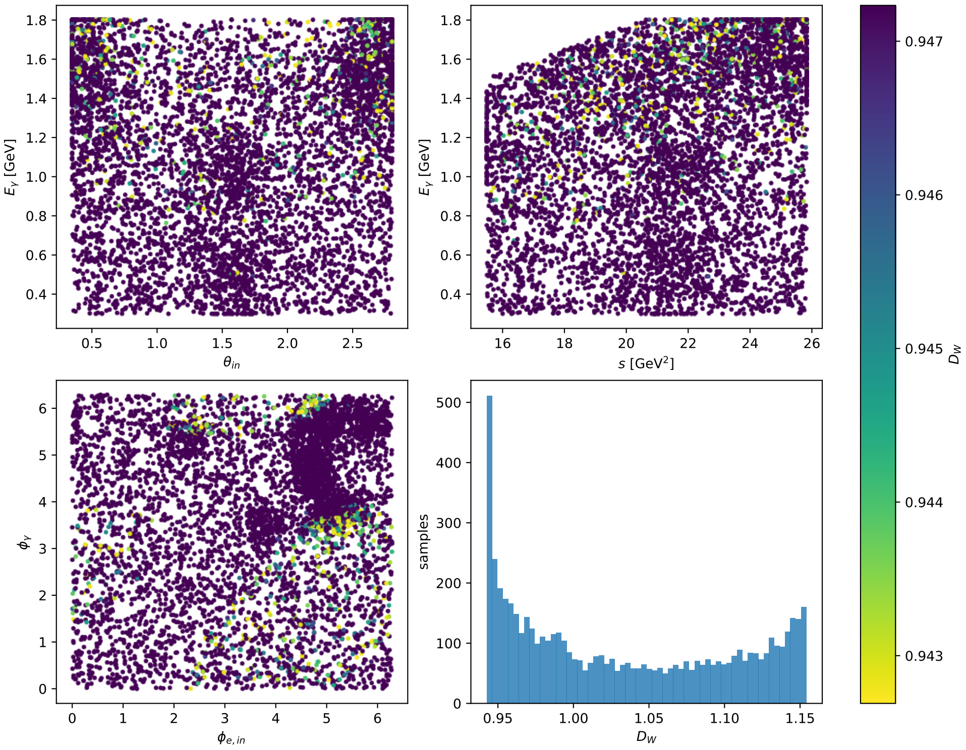
Expanded W search: L electron + Tx proton [LTx], min D_W=0.94269
