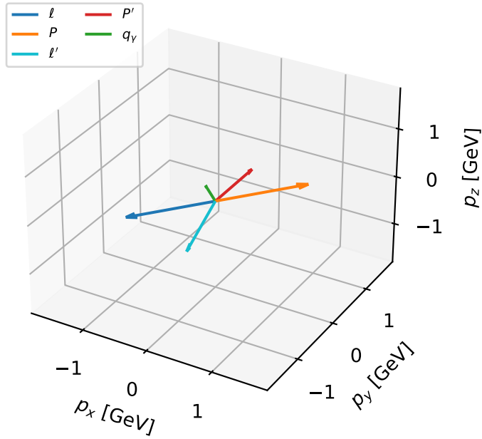
3D momenta
