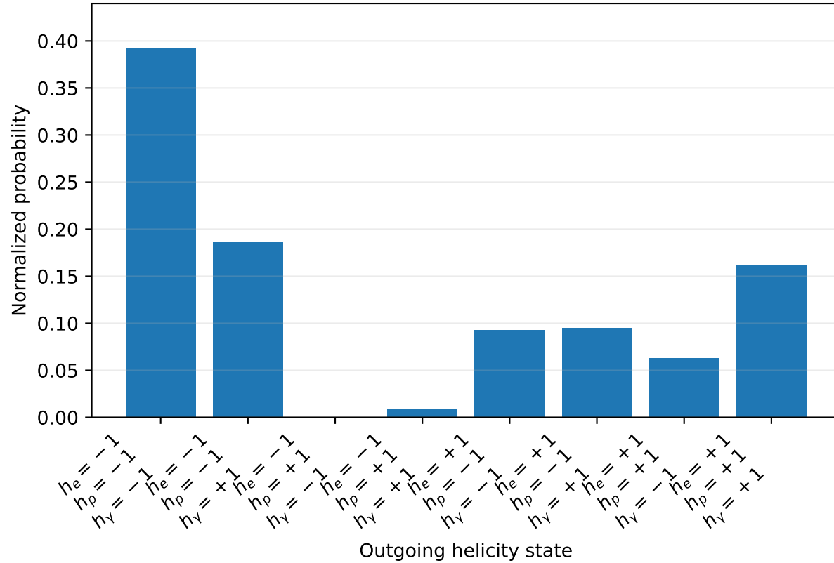
Outgoing helicity decomposition
