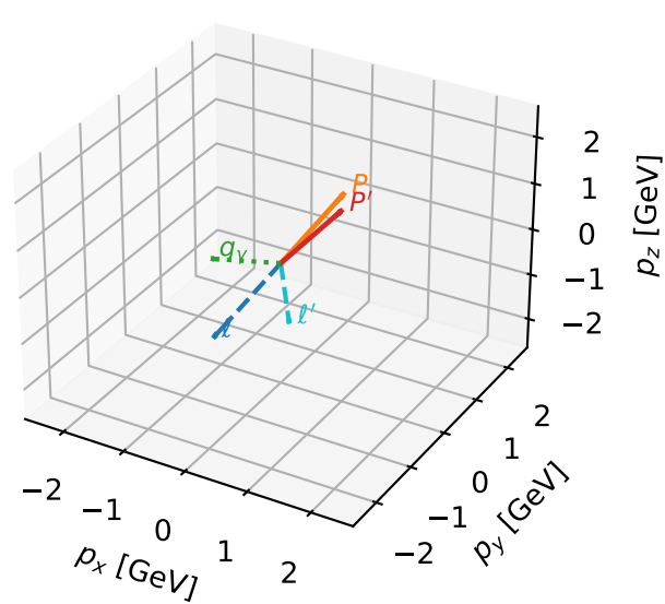
3D momenta
