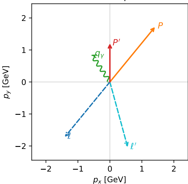
Transverse plane
