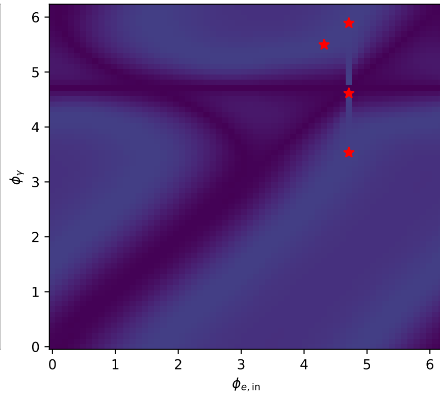
high_Egamma
