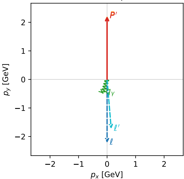
Transverse plane
