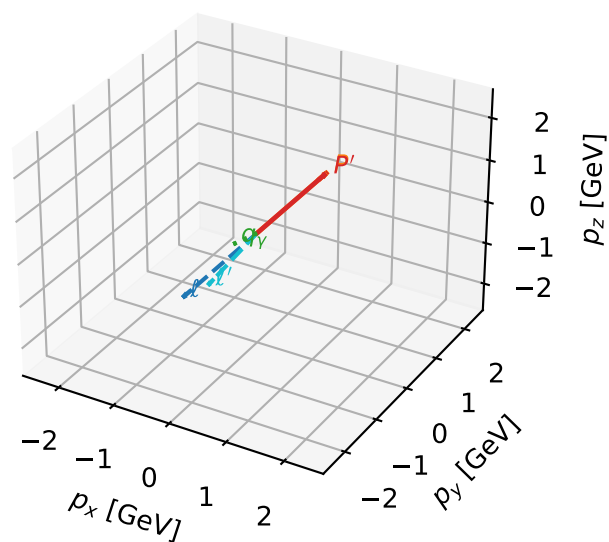
3D momenta
