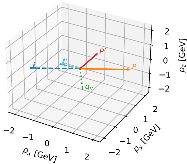
3D momenta
