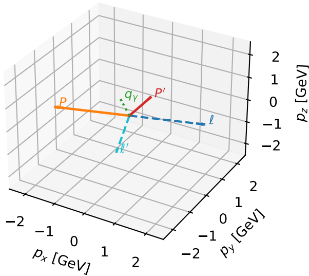
3D momenta
