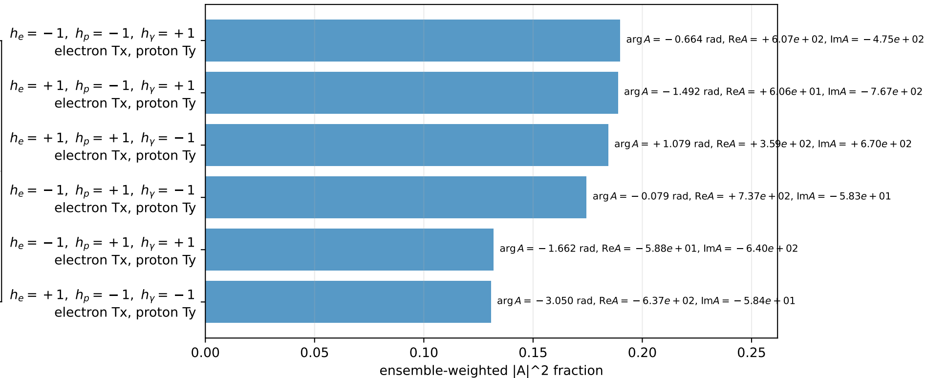
Leading helicity components and complex phases
