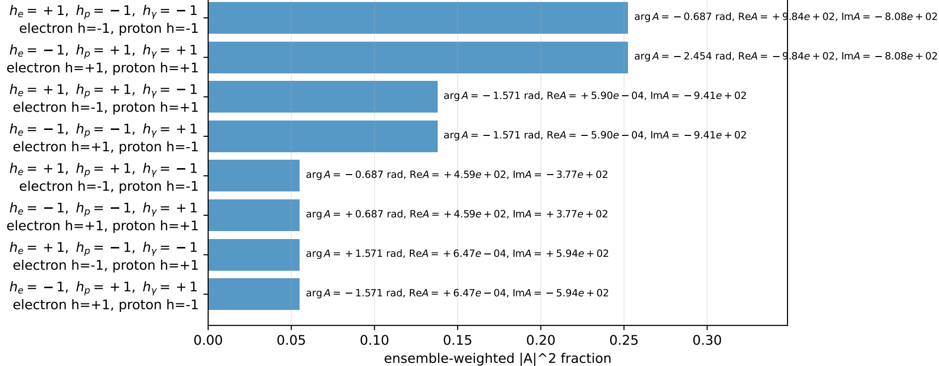
Leading helicity components and complex phases
