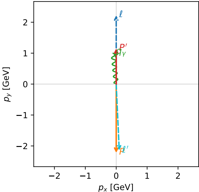
Transverse plane
