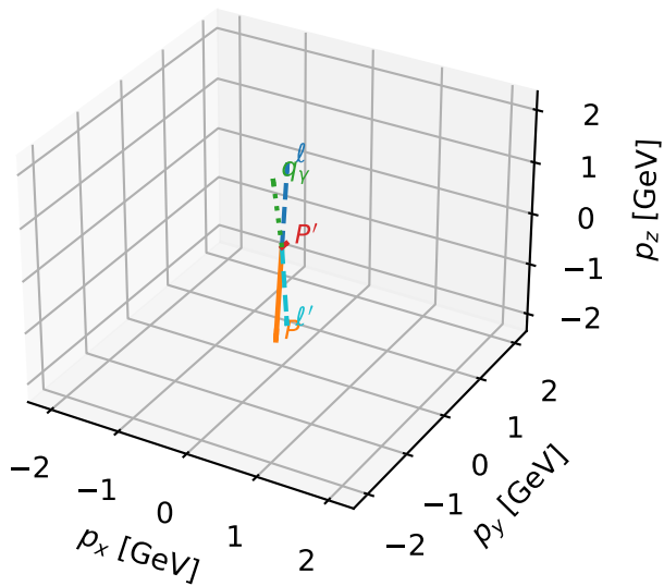
3D momenta
