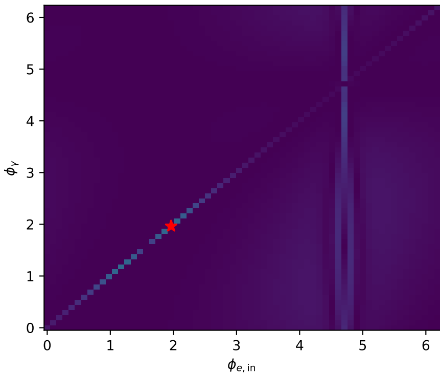
high_s_high_theta_in_low_Egamma min D_W=0.7607
