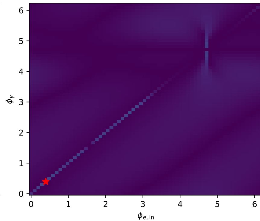
high_s_high_theta_in_high_Egamma min D_W=0.9084
