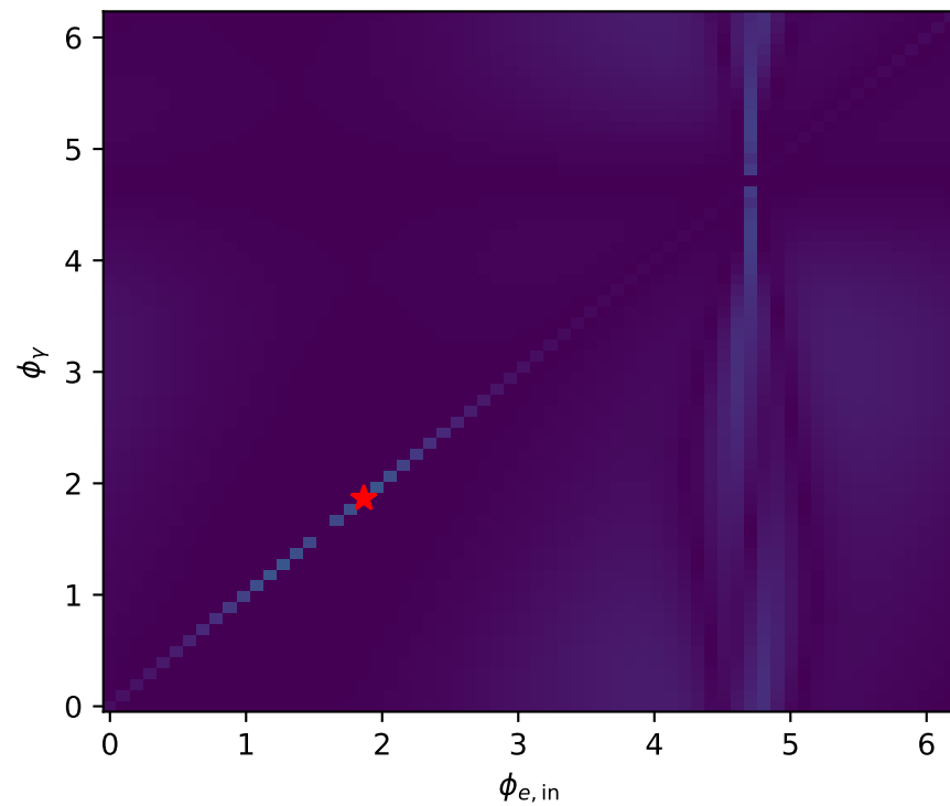
high_s_high_theta_in_mid_Egamma min D_W=0.8477
